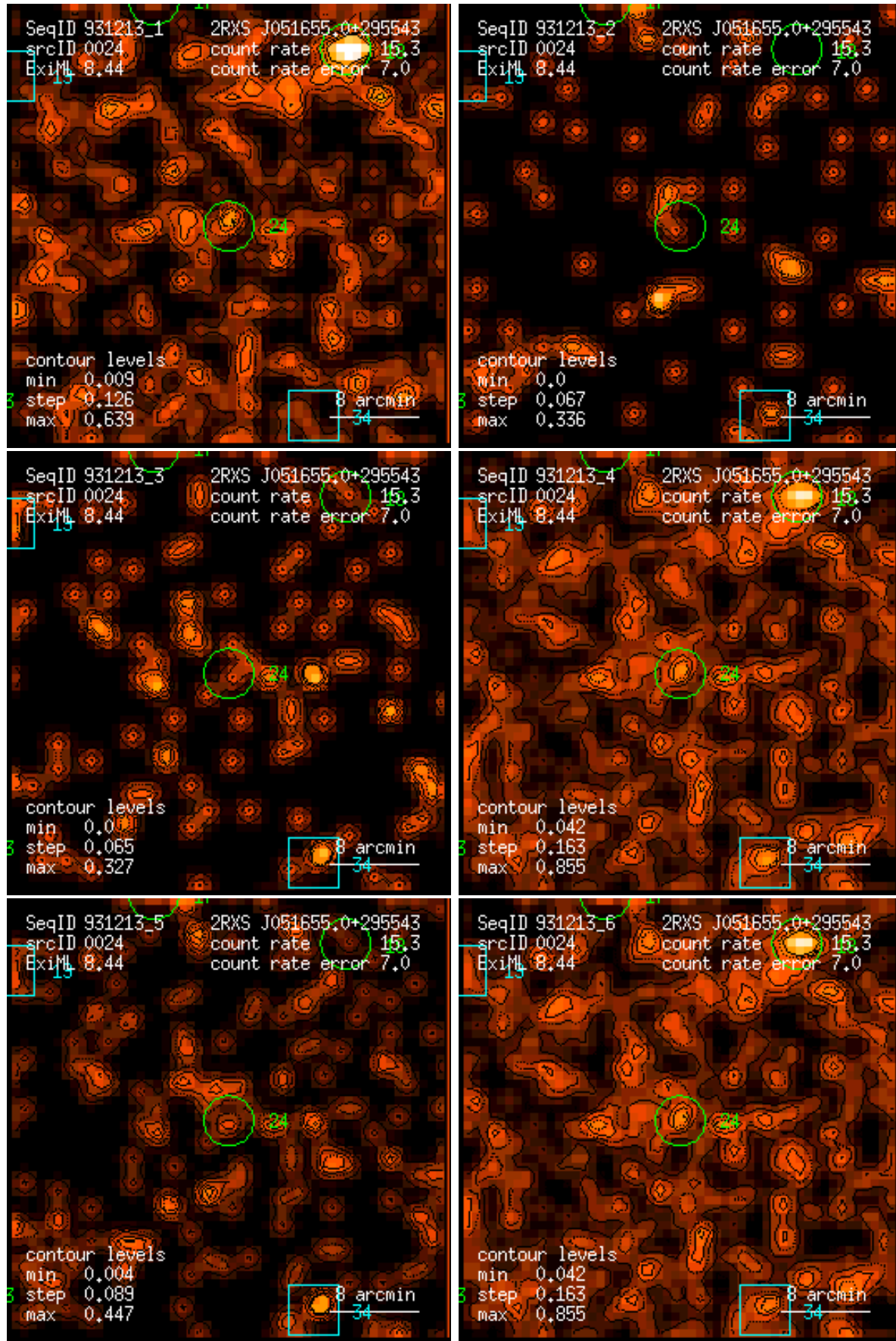
Figure 24: RASS 931213: detection 0024: band rate images, Gaussian filter: (1) PSPC channels 11 – 41, (2) 52 – 90, (3) 91 – 201, (4) 11 – 235, (5) 52 – 201, (6) 11 – 201. Broad band rates in counts/ks. Band rate contour levels in counts/ks/arcmin 2 .
