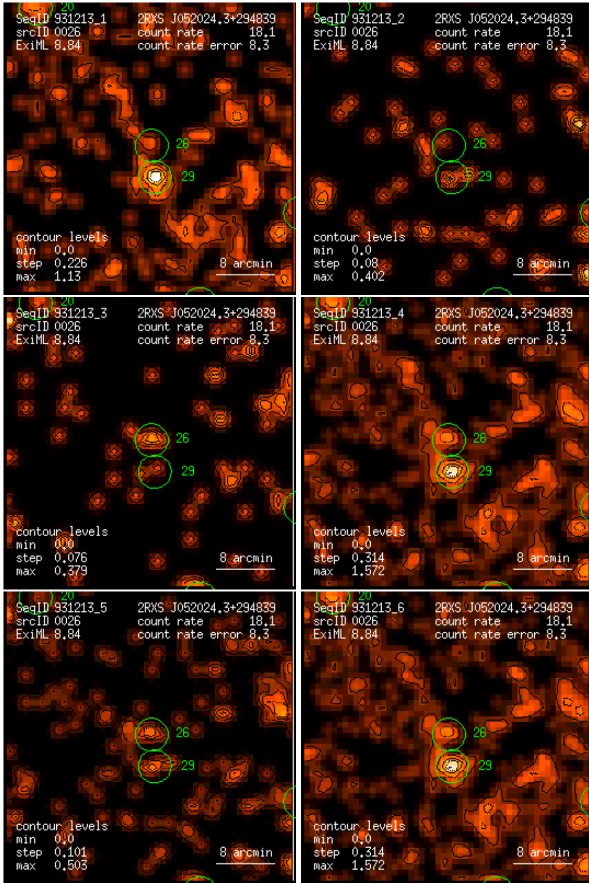
Figure 26: RASS 931213: detection 0026: band rate images, Gaussian filter: (1) PSPC channels 11 – 41, (2) 52 – 90, (3) 91 – 201, (4) 11 – 235, (5) 52 – 201, (6) 11 – 201. Broad band rates in counts/ks. Band rate contour levels in counts/ks/arcmin 2 .
