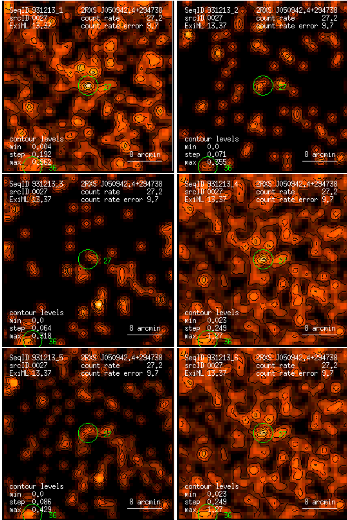
Figure 27: RASS 931213: detection 0027: band rate images, Gaussian filter: (1) PSPC channels 11 – 41, (2) 52 – 90, (3) 91 – 201, (4) 11 – 235, (5) 52 – 201, (6) 11 – 201. Broad band rates in counts/ks. Band rate contour levels in counts/ks/arcmin 2 .
