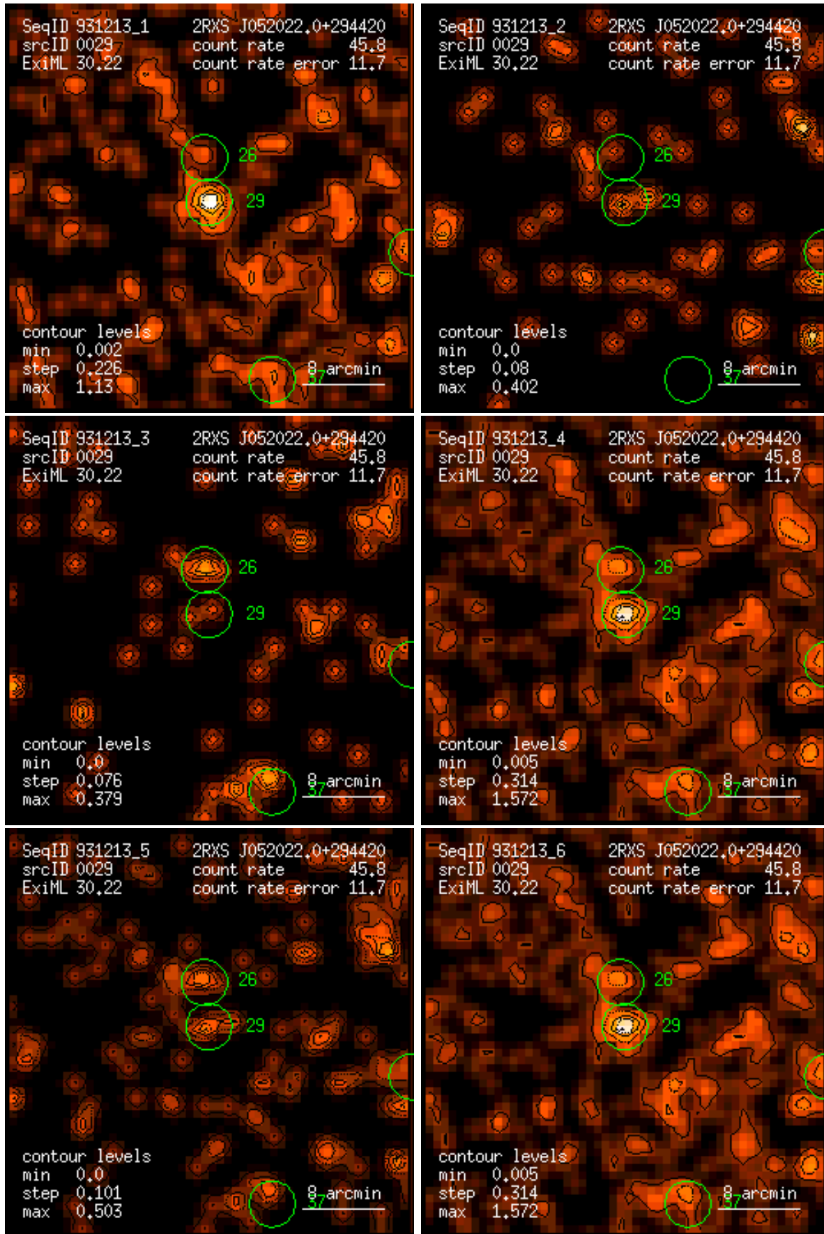
Figure 29: RASS 931213: detection 0029: band rate images, Gaussian filter: (1) PSPC channels 11 – 41, (2) 52 – 90, (3) 91 – 201, (4) 11 – 235, (5) 52 – 201, (6) 11 – 201. Broad band rates in counts/ks. Band rate contour levels in counts/ks/arcmin 2 .
