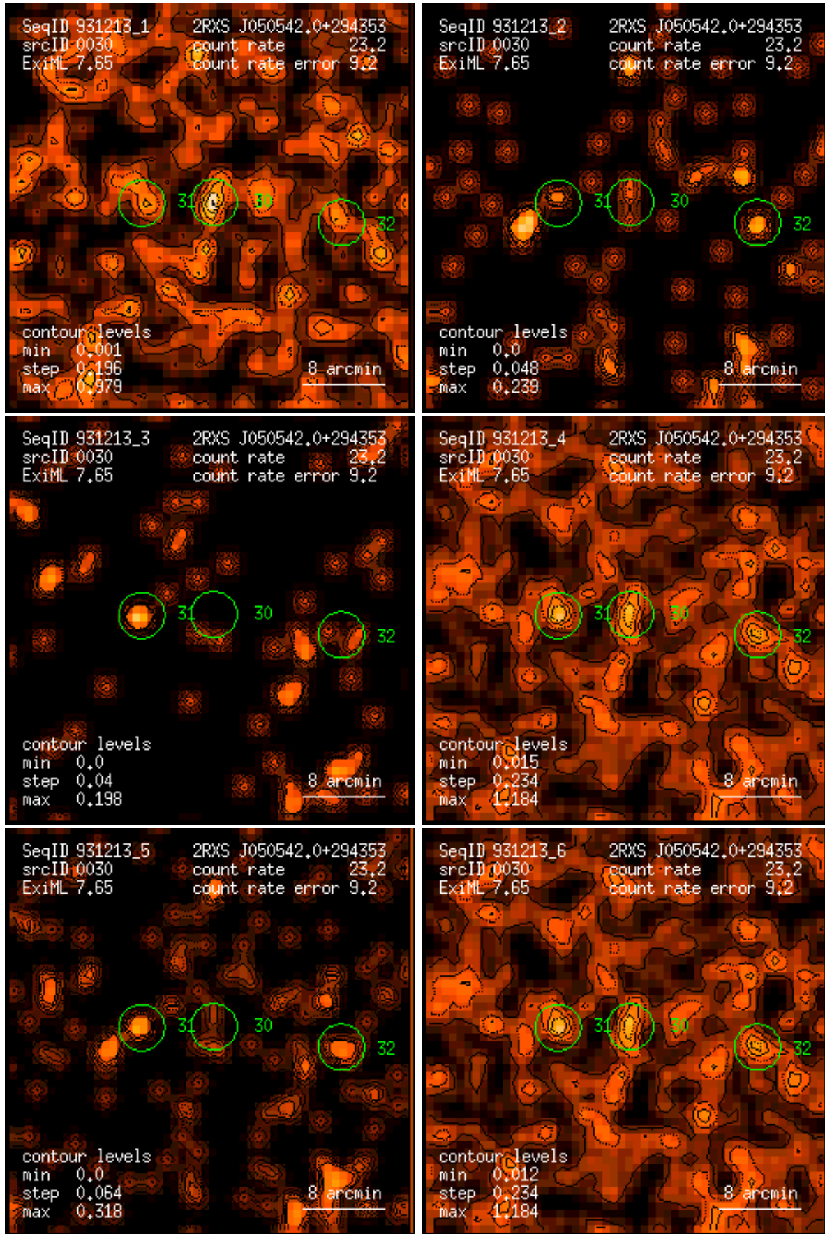
Figure 30: RASS 931213: detection 0030: band rate images, Gaussian filter: (1) PSPC channels 11 – 41, (2) 52 – 90, (3) 91 – 201, (4) 11 – 235, (5) 52 – 201, (6) 11 – 201. Broad band rates in counts/ks. Band rate contour levels in counts/ks/arcmin 2 .
