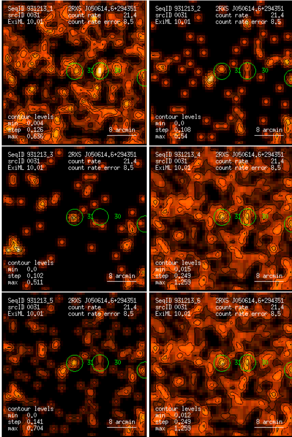
Figure 31: RASS 931213: detection 0031: band rate images, Gaussian filter: (1) PSPC channels 11 – 41, (2) 52 – 90, (3) 91 – 201, (4) 11 – 235, (5) 52 – 201, (6) 11 – 201. Broad band rates in counts/ks. Band rate contour levels in counts/ks/arcmin 2 .
