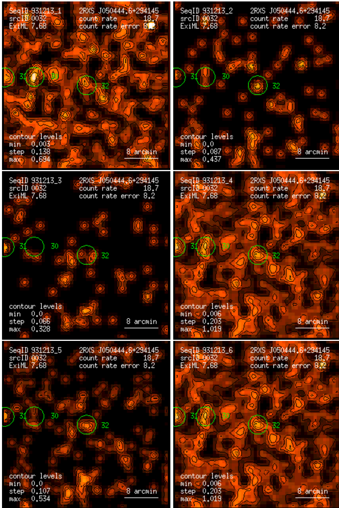
Figure 32: RASS 931213: detection 0032: band rate images, Gaussian filter: (1) PSPC channels 11 – 41, (2) 52 – 90, (3) 91 – 201, (4) 11 – 235, (5) 52 – 201, (6) 11 – 201. Broad band rates in counts/ks. Band rate contour levels in counts/ks/arcmin 2 .
