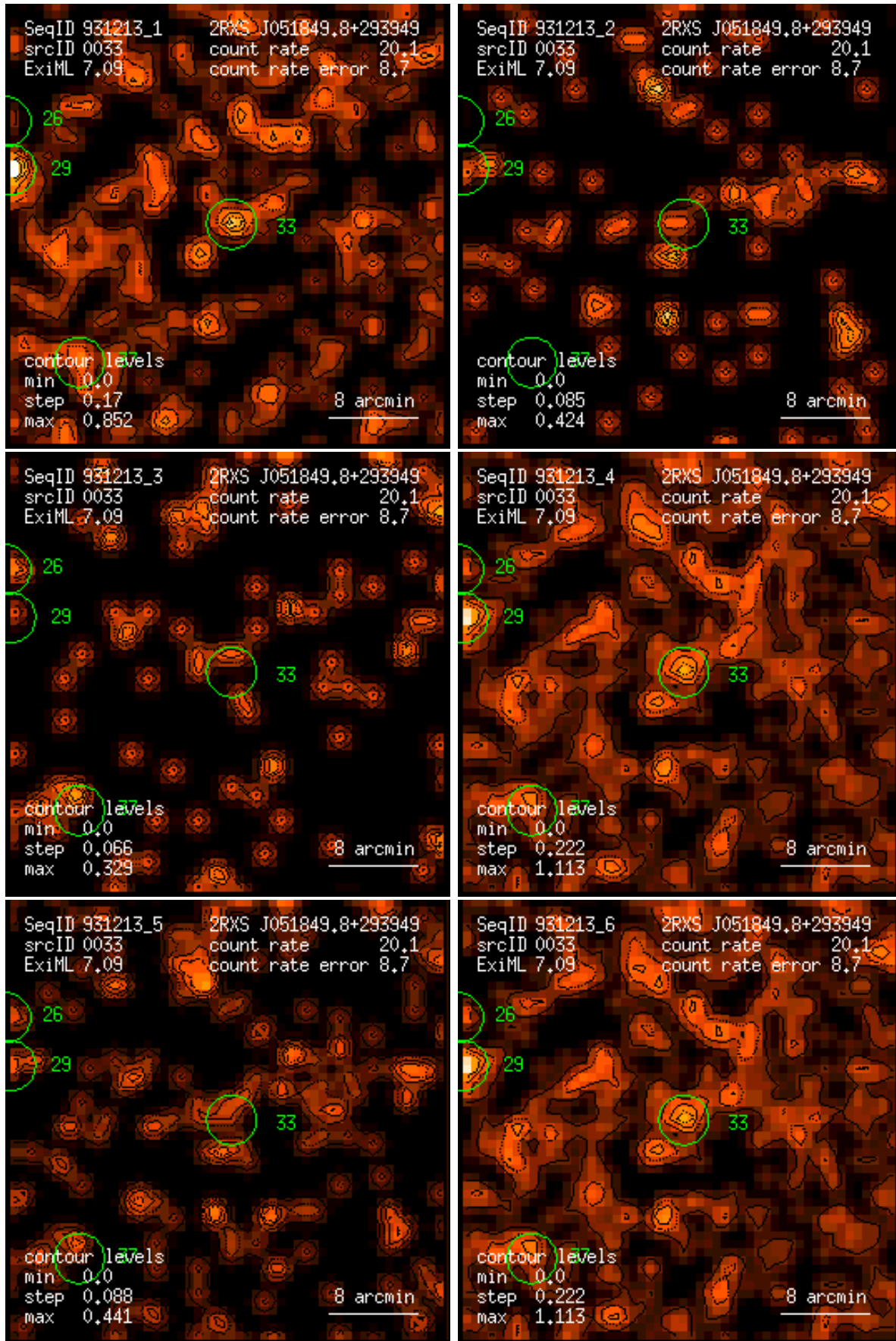
Figure 33: RASS 931213: detection 0033: band rate images, Gaussian filter: (1) PSPC channels 11 – 41, (2) 52 – 90, (3) 91 – 201, (4) 11 – 235, (5) 52 – 201, (6) 11 – 201. Broad band rates in counts/ks. Band rate contour levels in counts/ks/arcmin 2 .
