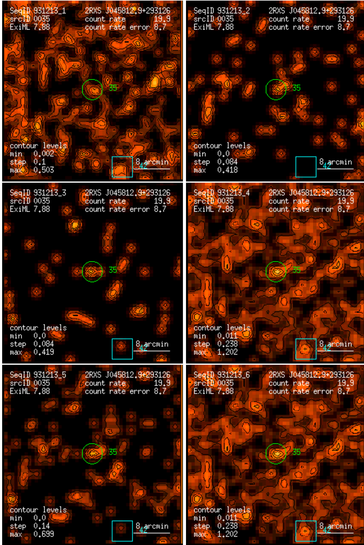
Figure 35: RASS 931213: detection 0035: band rate images, Gaussian filter: (1) PSPC channels 11 – 41, (2) 52 – 90, (3) 91 – 201, (4) 11 – 235, (5) 52 – 201, (6) 11 – 201. Broad band rates in counts/ks. Band rate contour levels in counts/ks/arcmin 2 .
