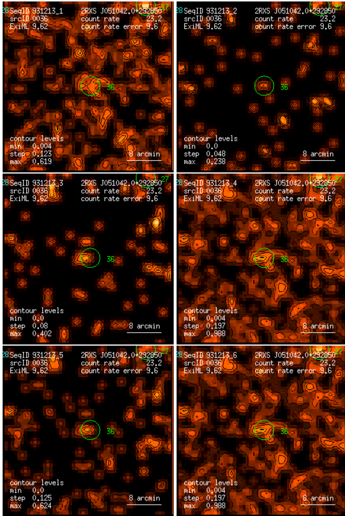
Figure 36: RASS 931213: detection 0036: band rate images, Gaussian filter: (1) PSPC channels 11 – 41, (2) 52 – 90, (3) 91 – 201, (4) 11 – 235, (5) 52 – 201, (6) 11 – 201. Broad band rates in counts/ks. Band rate contour levels in counts/ks/arcmin 2 .
