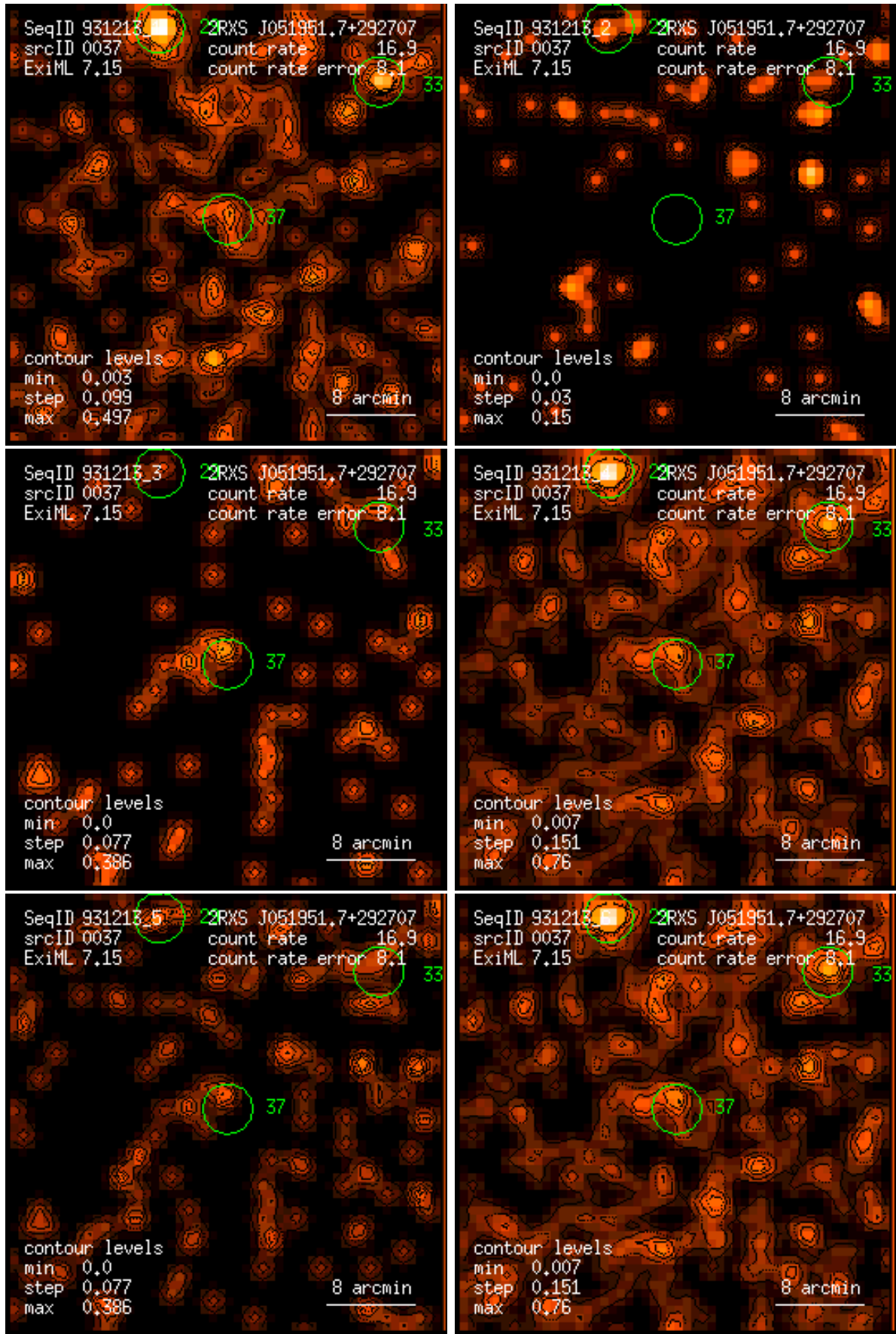
Figure 37: RASS 931213: detection 0037: band rate images, Gaussian filter: (1) PSPC channels 11 – 41, (2) 52 – 90, (3) 91 – 201, (4) 11 – 235, (5) 52 – 201, (6) 11 – 201. Broad band rates in counts/ks. Band rate contour levels in counts/ks/arcmin 2 .
