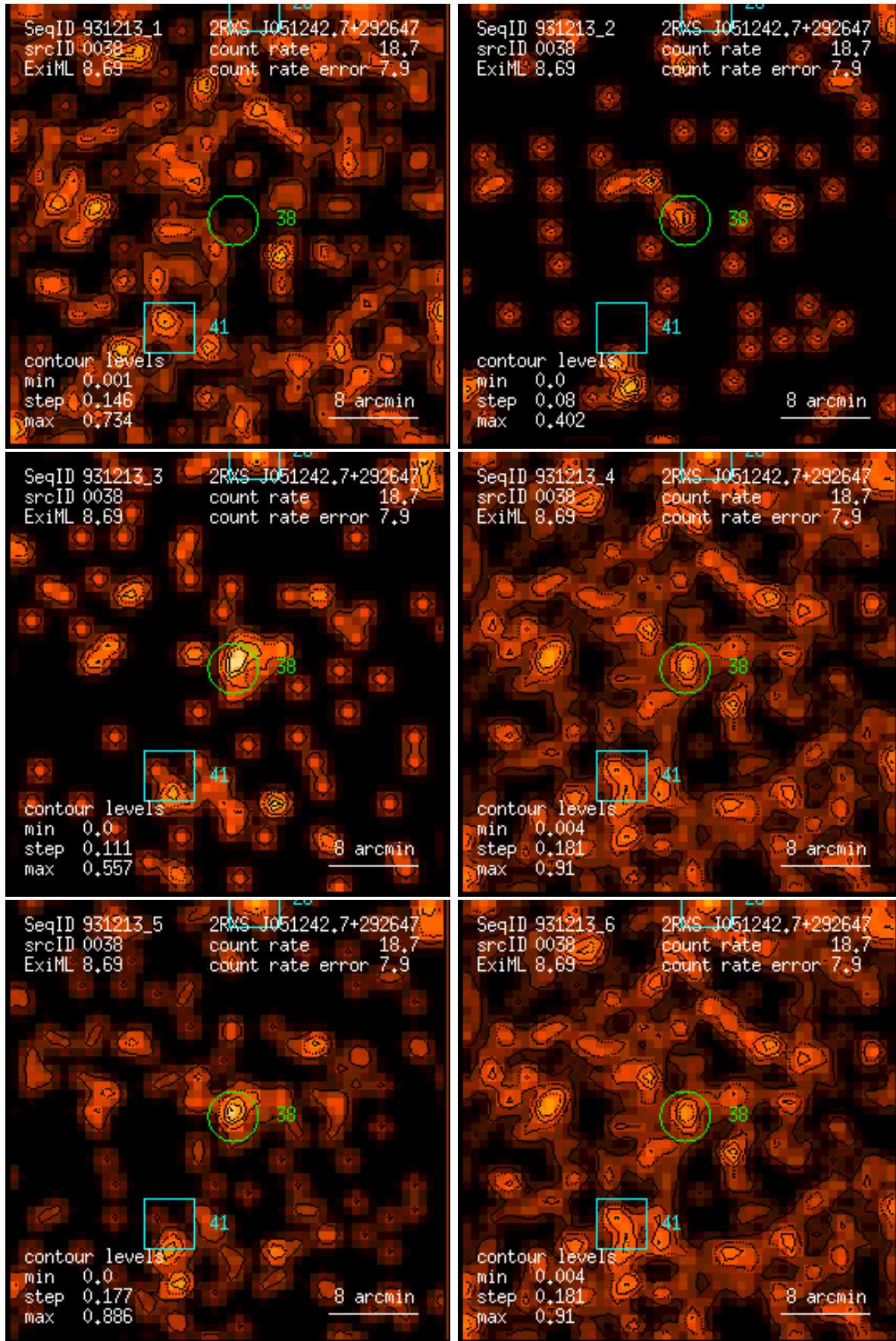
Figure 38: RASS 931213: detection 0038: band rate images, Gaussian filter: (1) PSPC channels 11 – 41, (2) 52 – 90, (3) 91 – 201, (4) 11 – 235, (5) 52 – 201, (6) 11 – 201. Broad band rates in counts/ks. Band rate contour levels in counts/ks/arcmin 2 .
