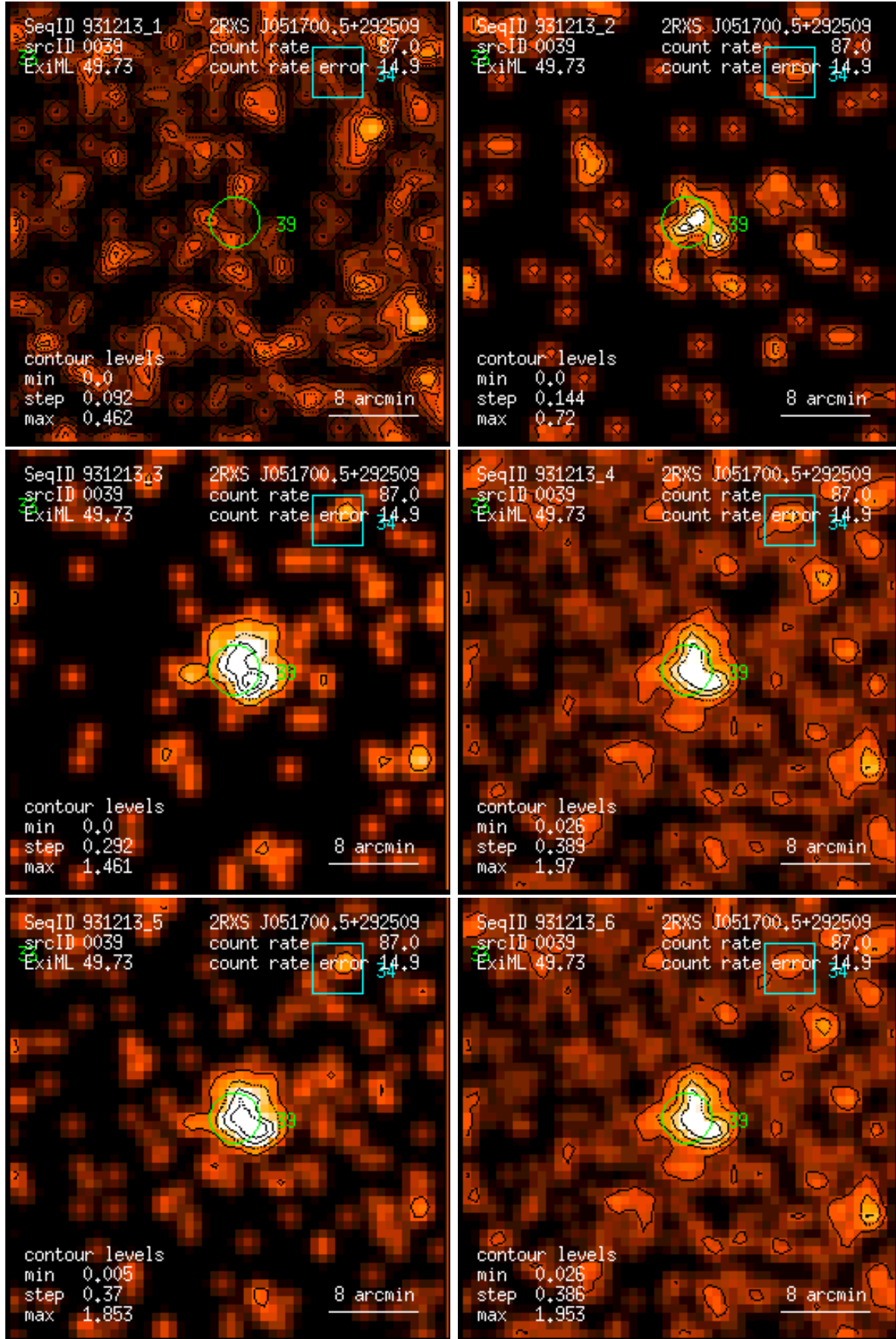
Figure 39: RASS 931213: detection 0039: band rate images, Gaussian filter: (1) PSPC channels 11 – 41, (2) 52 – 90, (3) 91 – 201, (4) 11 – 235, (5) 52 – 201, (6) 11 – 201. Broad band rates in counts/ks. Band rate contour levels in counts/ks/arcmin 2 .
