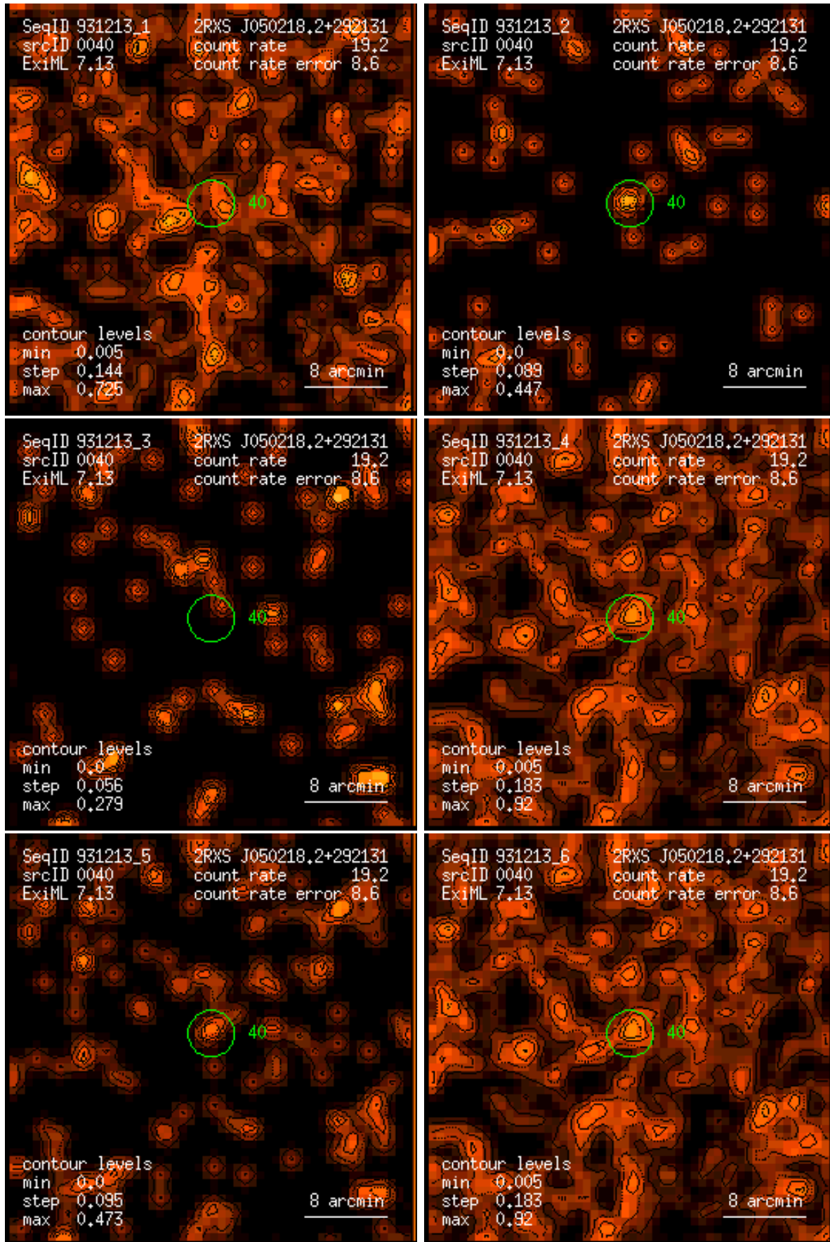
Figure 40: RASS 931213: detection 0040: band rate images, Gaussian filter: (1) PSPC channels 11 – 41, (2) 52 – 90, (3) 91 – 201, (4) 11 – 235, (5) 52 – 201, (6) 11 – 201. Broad band rates in counts/ks. Band rate contour levels in counts/ks/arcmin 2 .
