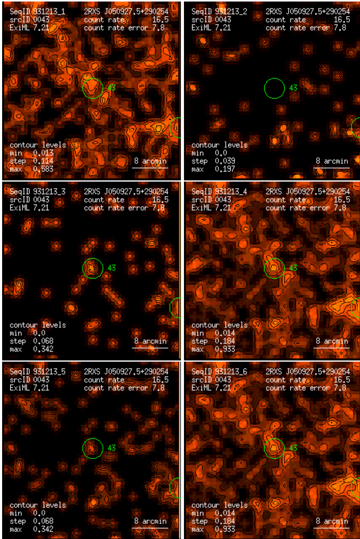
Figure 43: RASS 931213: detection 0043: band rate images, Gaussian filter: (1) PSPC channels 11 – 41, (2) 52 – 90, (3) 91 – 201, (4) 11 – 235, (5) 52 – 201, (6) 11 – 201. Broad band rates in counts/ks. Band rate contour levels in counts/ks/arcmin 2 .
