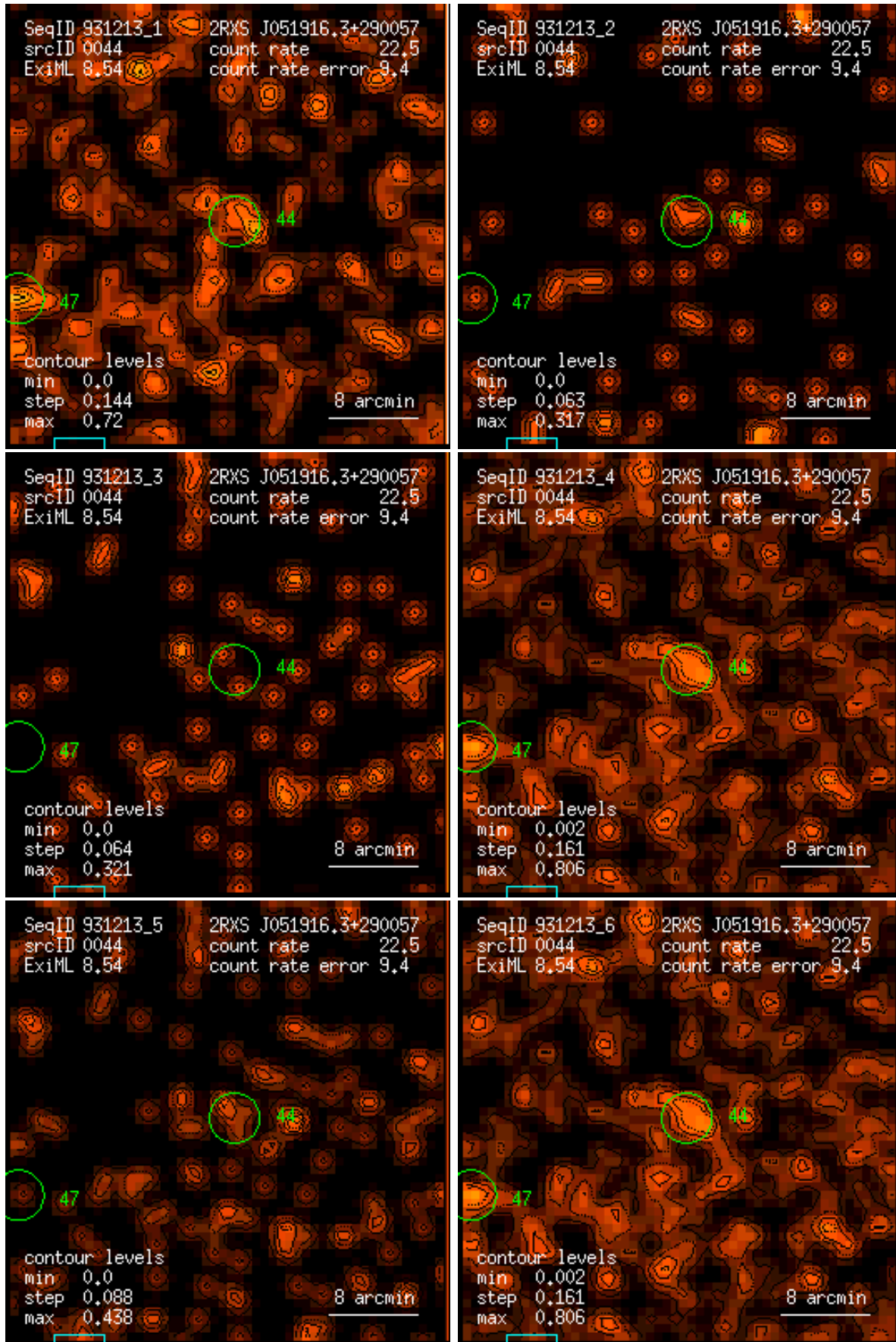
Figure 44: RASS 931213: detection 0044: band rate images, Gaussian filter: (1) PSPC channels 11 – 41, (2) 52 – 90, (3) 91 – 201, (4) 11 – 235, (5) 52 – 201, (6) 11 – 201. Broad band rates in counts/ks. Band rate contour levels in counts/ks/arcmin 2 .
