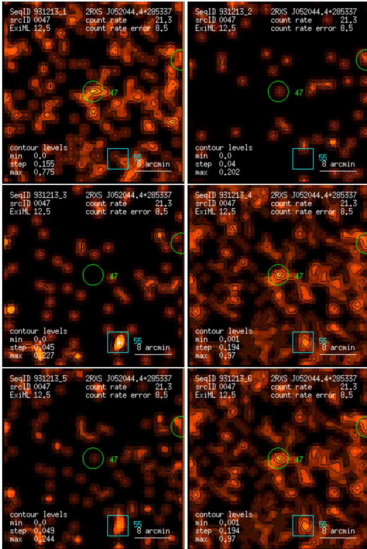
Figure 47: RASS 931213: detection 0047: band rate images, Gaussian filter: (1) PSPC channels 11 – 41, (2) 52 – 90, (3) 91 – 201, (4) 11 – 235, (5) 52 – 201, (6) 11 – 201. Broad band rates in counts/ks. Band rate contour levels in counts/ks/arcmin 2 .
