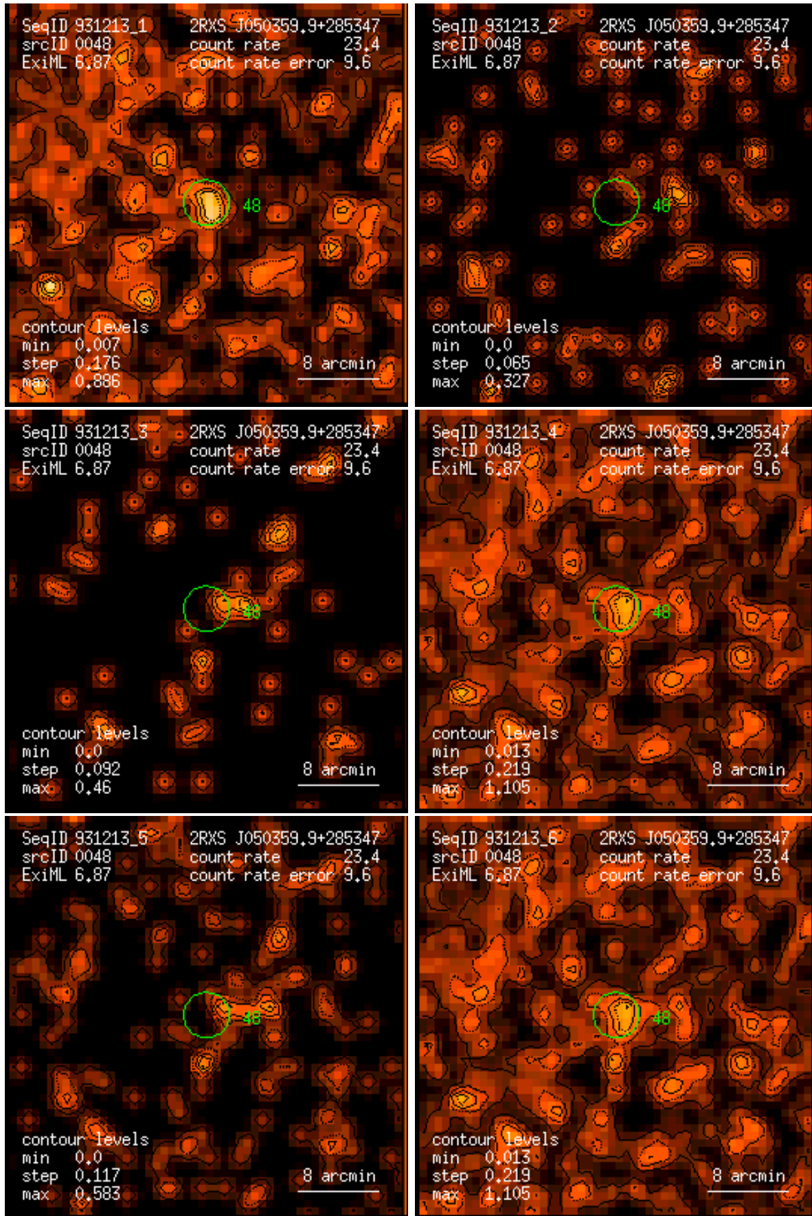
Figure 48: RASS 931213: detection 0048: band rate images, Gaussian filter: (1) PSPC channels 11 – 41, (2) 52 – 90, (3) 91 – 201, (4) 11 – 235, (5) 52 – 201, (6) 11 – 201. Broad band rates in counts/ks. Band rate contour levels in counts/ks/arcmin 2 .
