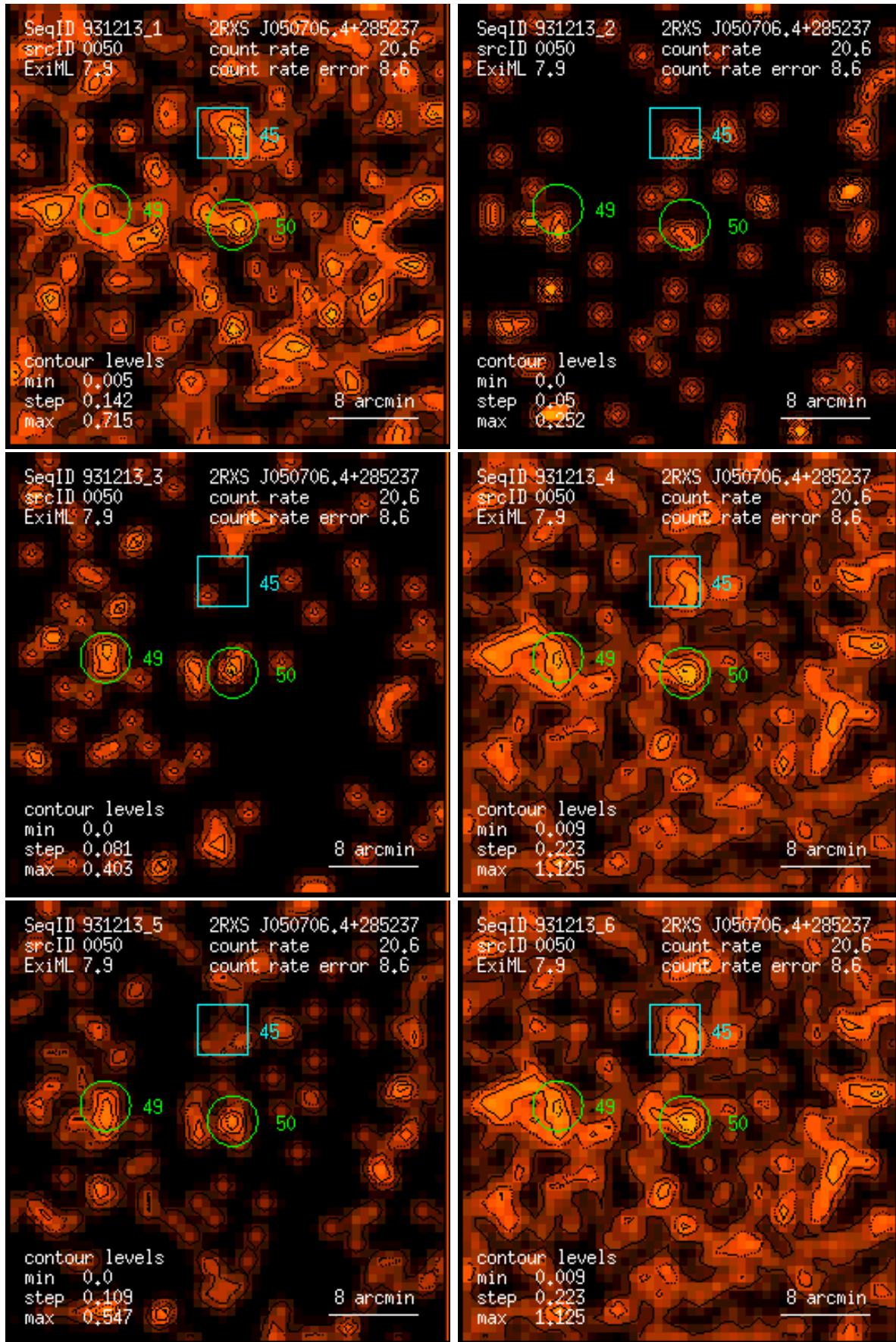
Figure 50: RASS 931213: detection 0050: band rate images, Gaussian filter: (1) PSPC channels 11 – 41, (2) 52 – 90, (3) 91 – 201, (4) 11 – 235, (5) 52 – 201, (6) 11 – 201. Broad band rates in counts/ks. Band rate contour levels in counts/ks/arcmin 2 .
