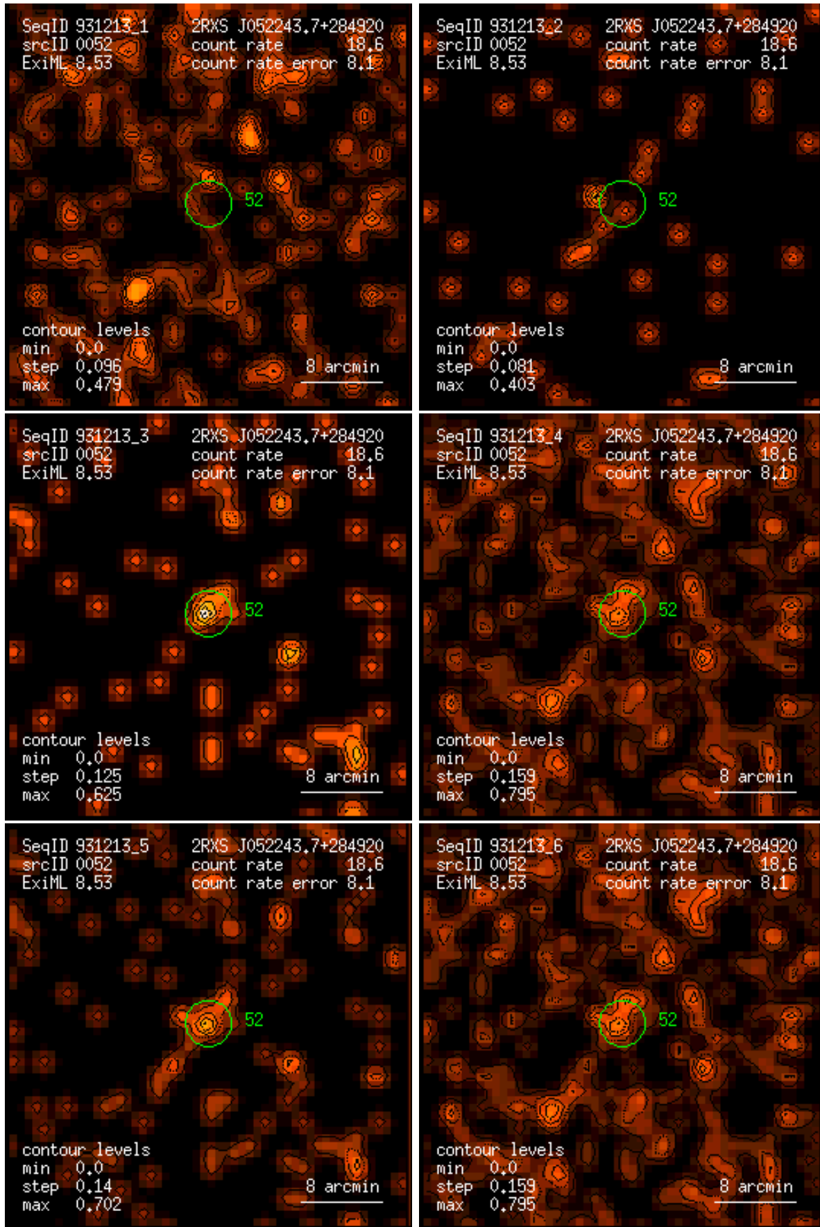
Figure 52: RASS 931213: detection 0052: band rate images, Gaussian filter: (1) PSPC channels 11 – 41, (2) 52 – 90, (3) 91 – 201, (4) 11 – 235, (5) 52 – 201, (6) 11 – 201. Broad band rates in counts/ks. Band rate contour levels in counts/ks/arcmin 2 .
