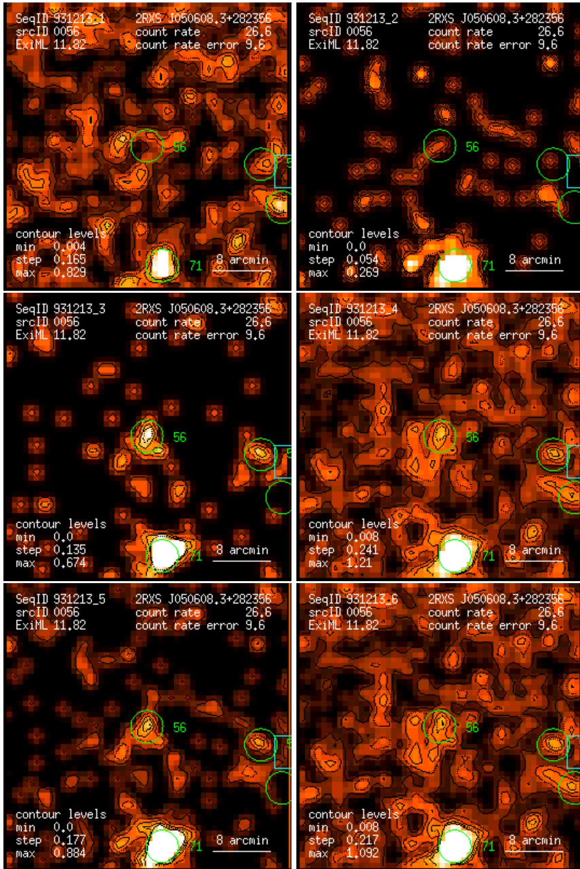
Figure 56: RASS 931213: detection 0056: band rate images, Gaussian filter: (1) PSPC channels 11 – 41, (2) 52 – 90, (3) 91 – 201, (4) 11 – 235, (5) 52 – 201, (6) 11 – 201. Broad band rates in counts/ks. Band rate contour levels in counts/ks/arcmin 2 .
