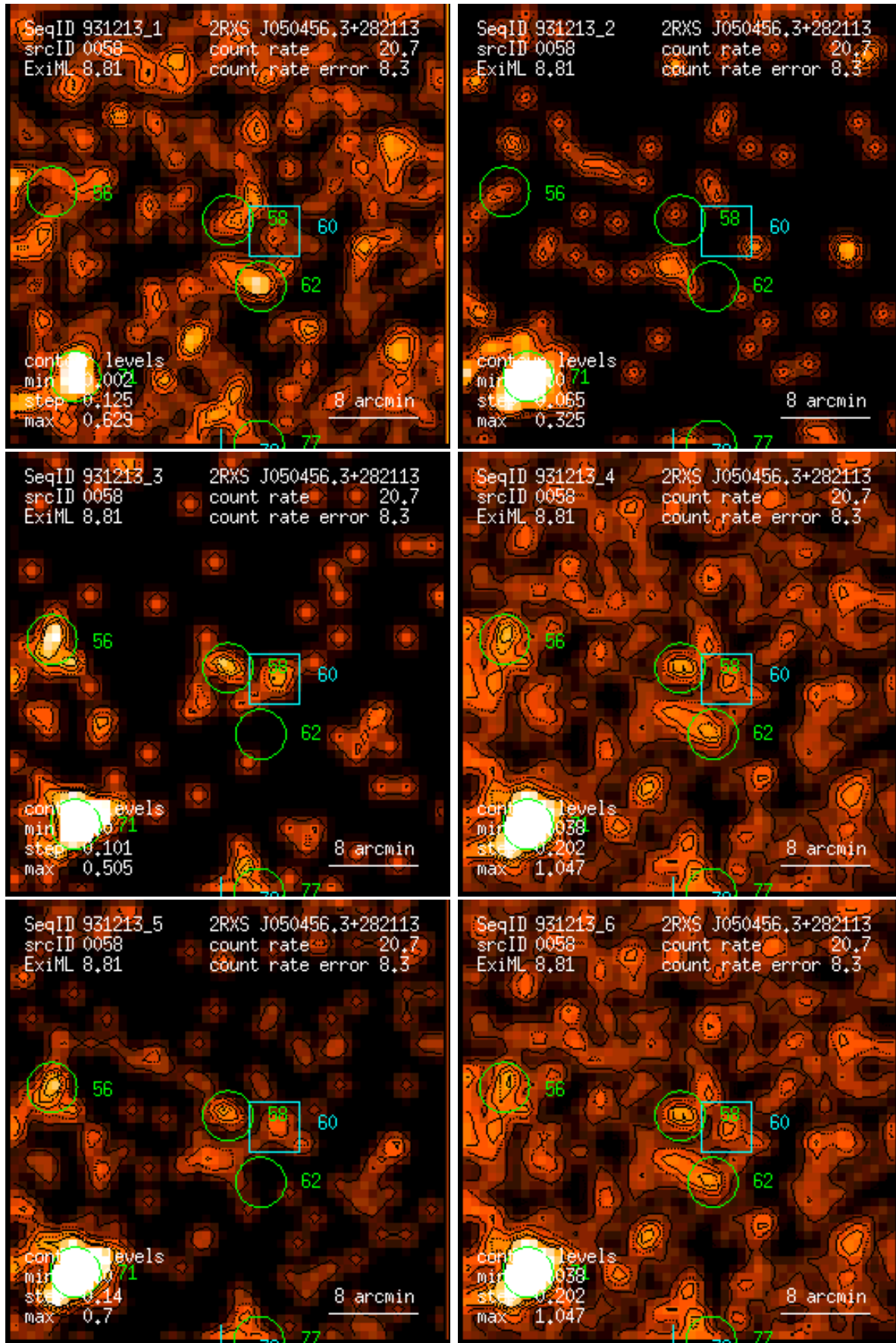
Figure 58: RASS 931213: detection 0058: band rate images, Gaussian filter: (1) PSPC channels 11 – 41, (2) 52 – 90, (3) 91 – 201, (4) 11 – 235, (5) 52 – 201, (6) 11 – 201. Broad band rates in counts/ks. Band rate contour levels in counts/ks/arcmin 2 .
