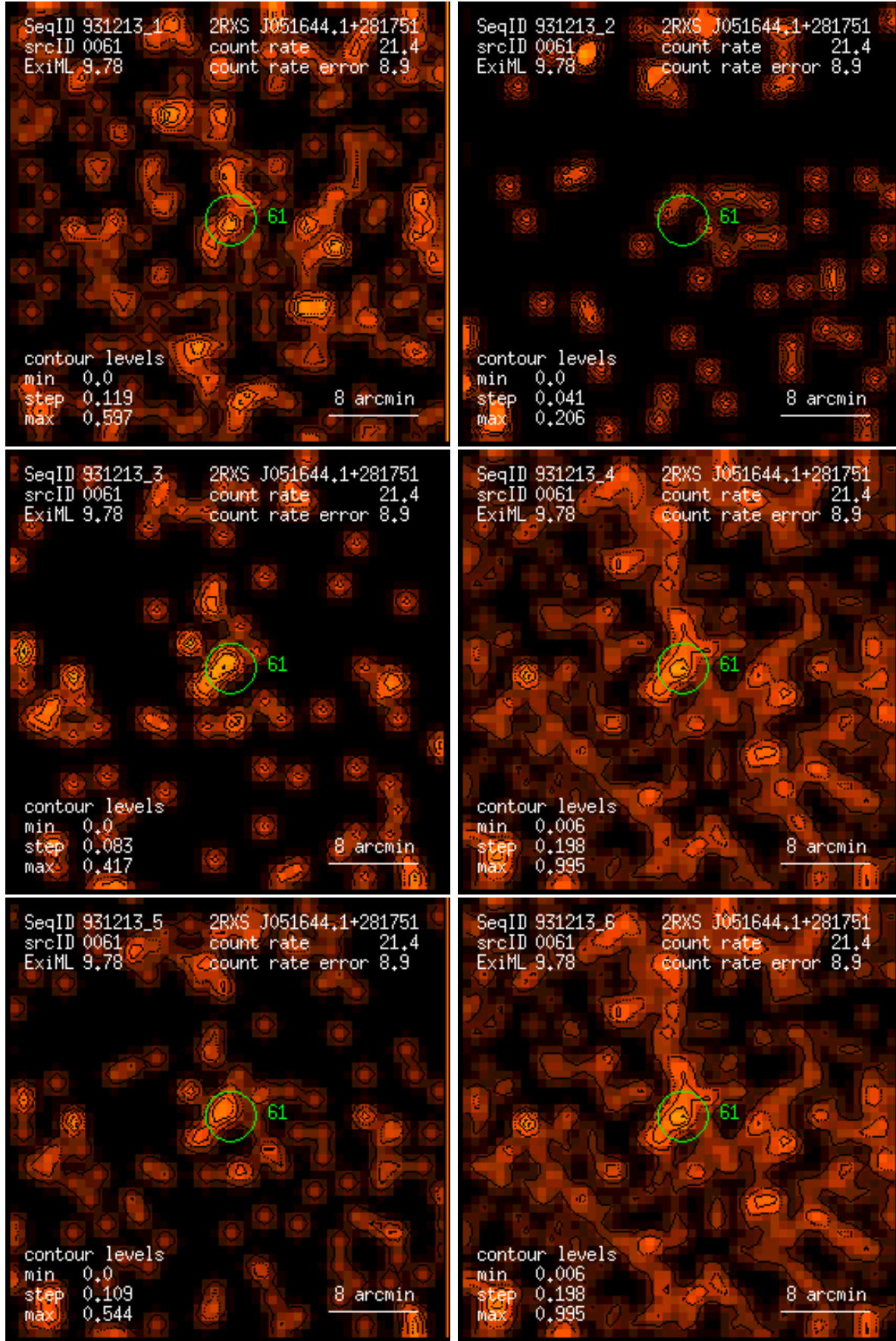
Figure 61: RASS 931213: detection 0061: band rate images, Gaussian filter: (1) PSPC channels 11 – 41, (2) 52 – 90, (3) 91 – 201, (4) 11 – 235, (5) 52 – 201, (6) 11 – 201. Broad band rates in counts/ks. Band rate contour levels in counts/ks/arcmin 2 .
