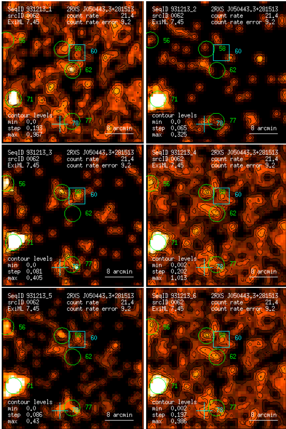
Figure 62: RASS 931213: detection 0062: band rate images, Gaussian filter: (1) PSPC channels 11 – 41, (2) 52 – 90, (3) 91 – 201, (4) 11 – 235, (5) 52 – 201, (6) 11 – 201. Broad band rates in counts/ks. Band rate contour levels in counts/ks/arcmin 2 .
