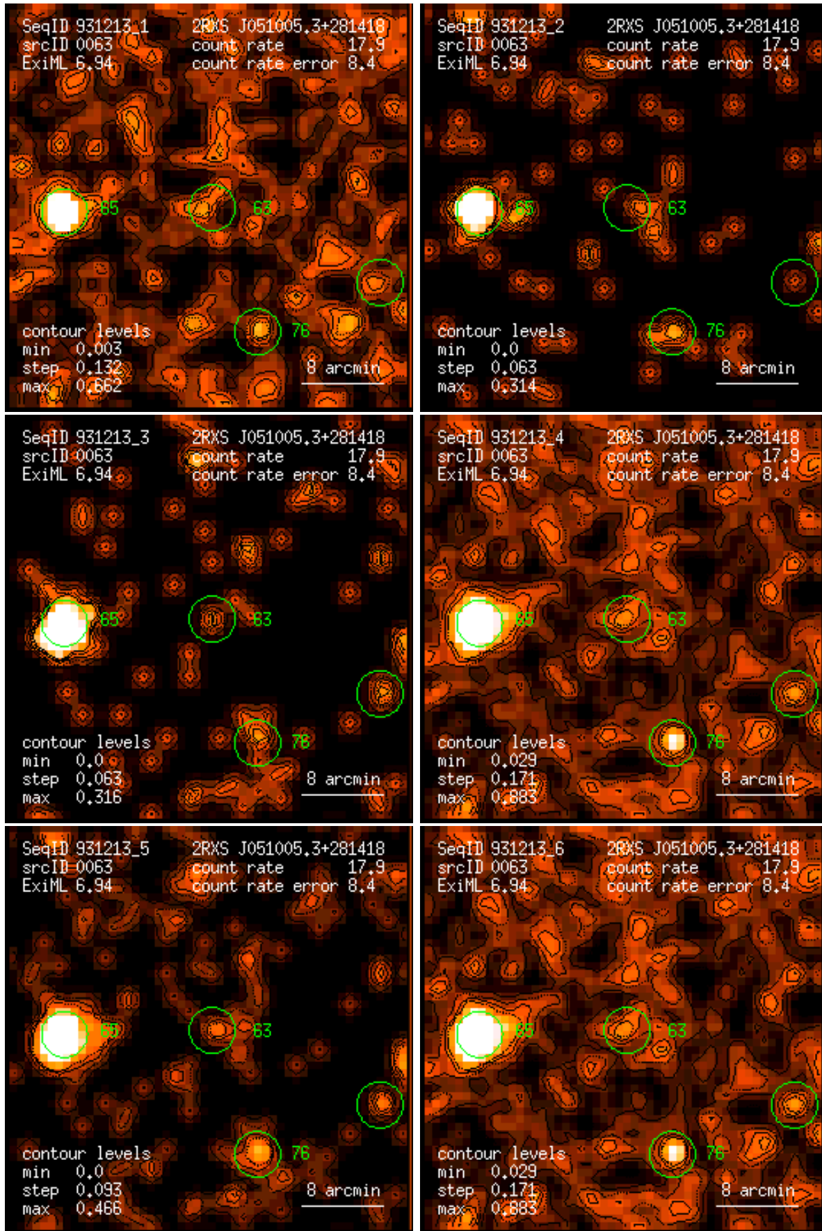
Figure 63: RASS 931213: detection 0063: band rate images, Gaussian filter: (1) PSPC channels 11 – 41, (2) 52 – 90, (3) 91 – 201, (4) 11 – 235, (5) 52 – 201, (6) 11 – 201. Broad band rates in counts/ks. Band rate contour levels in counts/ks/arcmin 2 .
