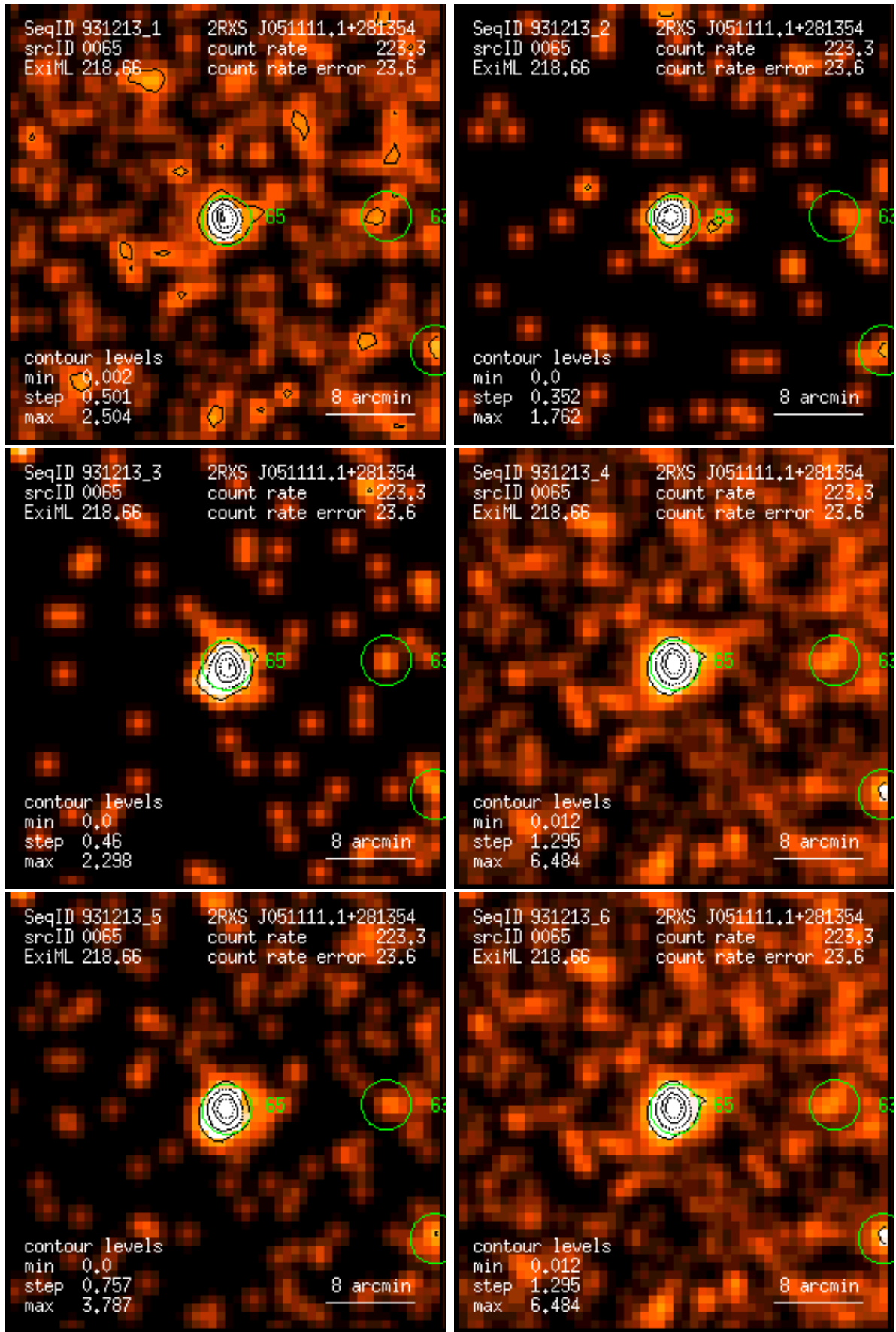
Figure 65: RASS 931213: detection 0065: band rate images, Gaussian filter: (1) PSPC channels 11 – 41, (2) 52 – 90, (3) 91 – 201, (4) 11 – 235, (5) 52 – 201, (6) 11 – 201. Broad band rates in counts/ks. Band rate contour levels in counts/ks/arcmin 2 .
