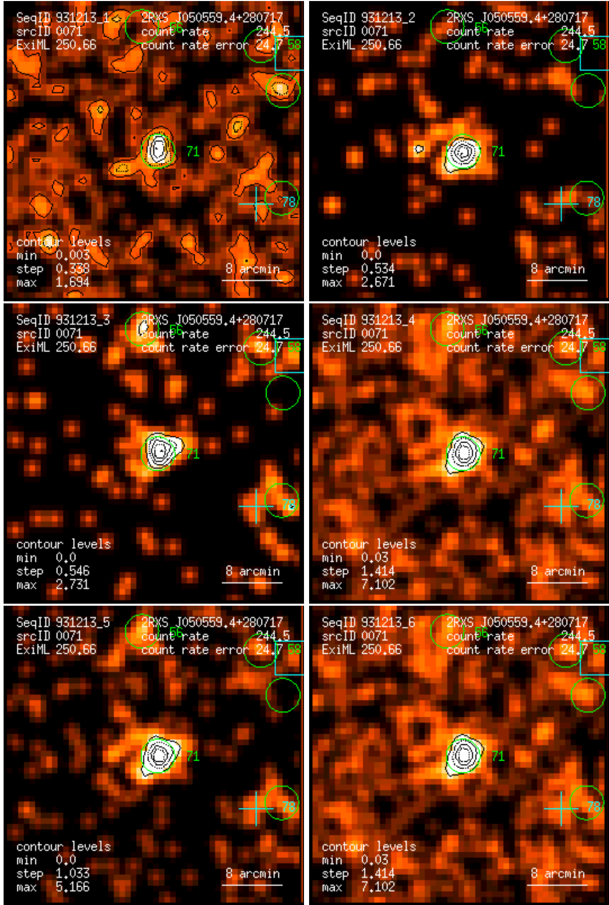
Figure 71: RASS 931213: detection 0071: band rate images, Gaussian filter: (1) PSPC channels 11 – 41, (2) 52 – 90, (3) 91 – 201, (4) 11 – 235, (5) 52 – 201, (6) 11 – 201. Broad band rates in counts/ks. Band rate contour levels in counts/ks/arcmin 2 .
