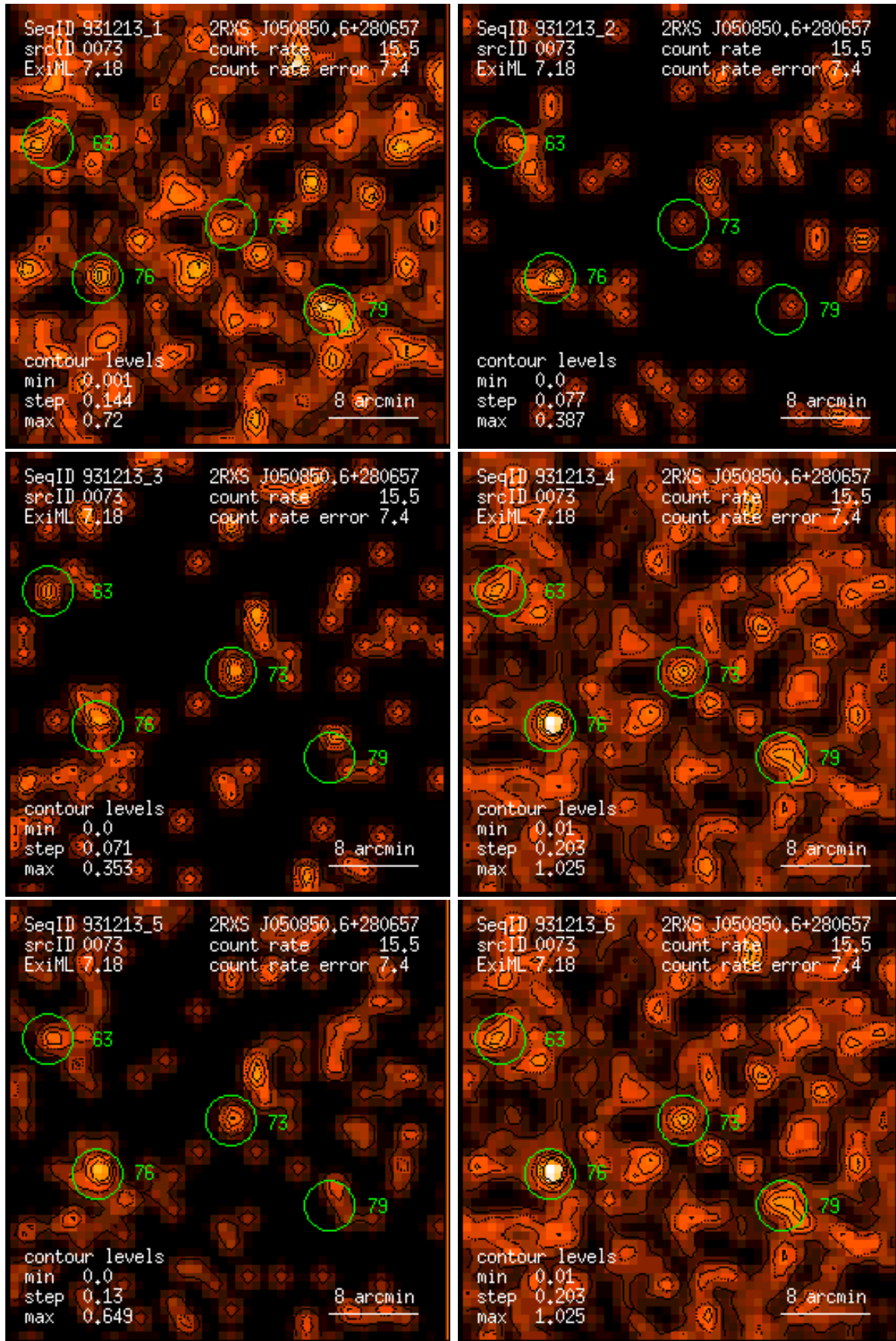
Figure 73: RASS 931213: detection 0073: band rate images, Gaussian filter: (1) PSPC channels 11 – 41, (2) 52 – 90, (3) 91 – 201, (4) 11 – 235, (5) 52 – 201, (6) 11 – 201. Broad band rates in counts/ks. Band rate contour levels in counts/ks/arcmin 2 .
