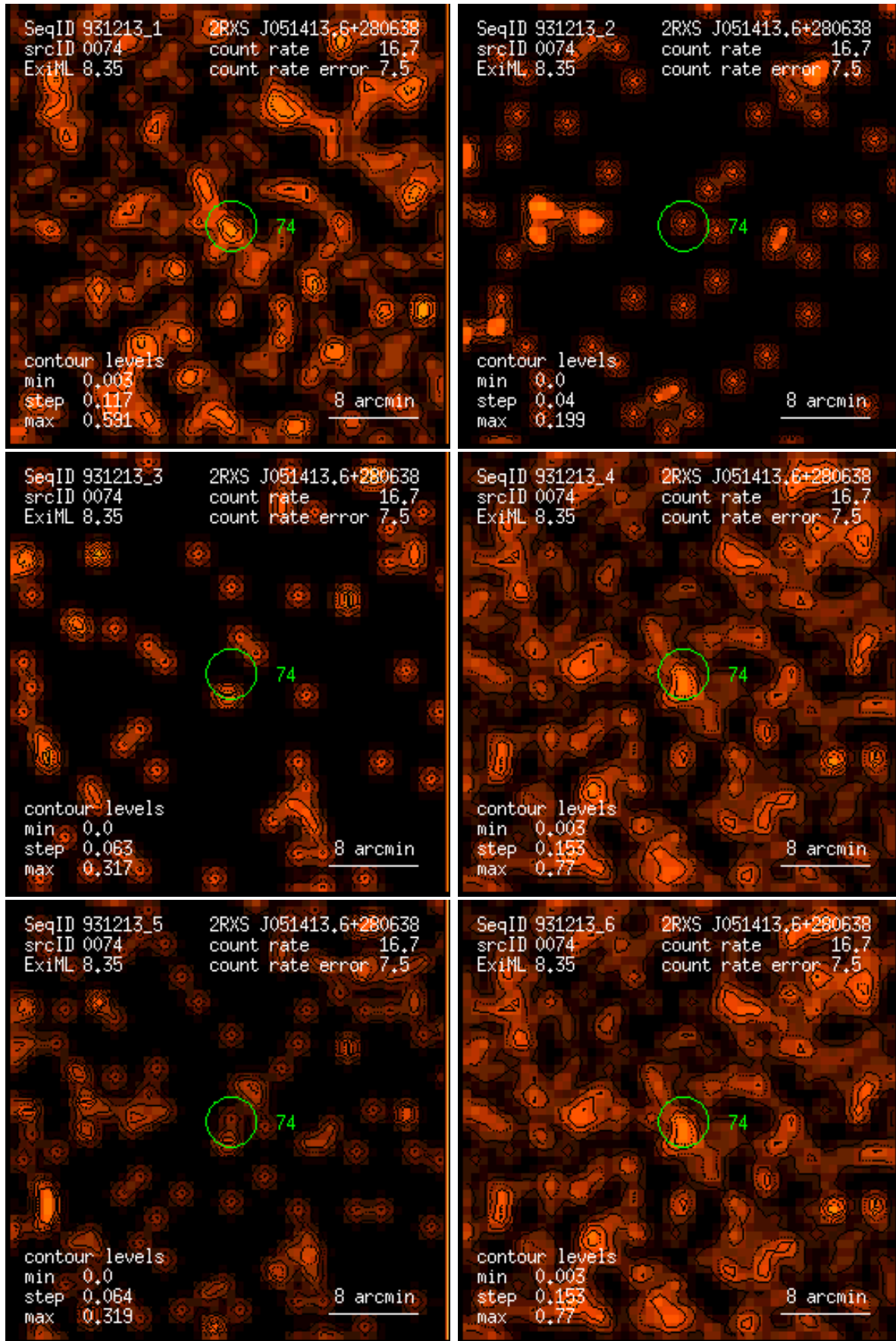
Figure 74: RASS 931213: detection 0074: band rate images, Gaussian filter: (1) PSPC channels 11 – 41, (2) 52 – 90, (3) 91 – 201, (4) 11 – 235, (5) 52 – 201, (6) 11 – 201. Broad band rates in counts/ks. Band rate contour levels in counts/ks/arcmin 2 .
