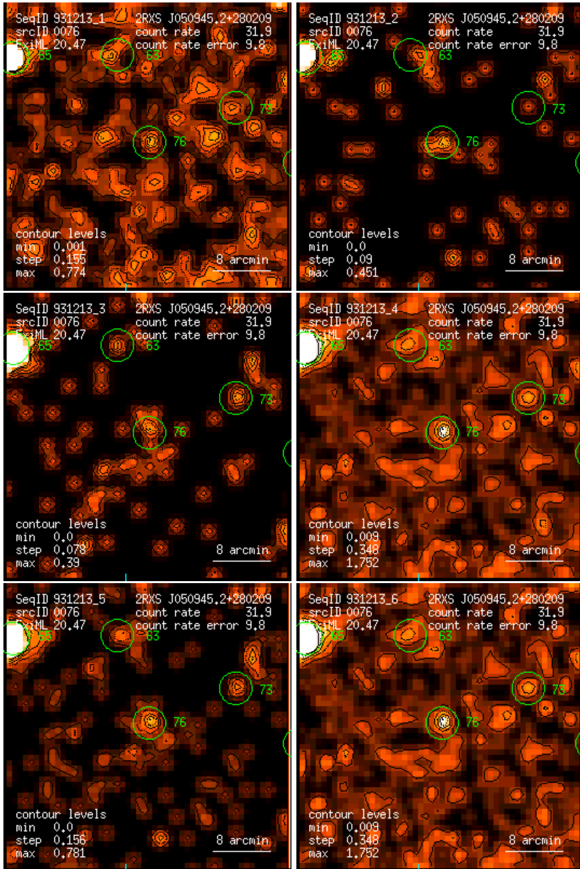
Figure 76: RASS 931213: detection 0076: band rate images, Gaussian filter: (1) PSPC channels 11 – 41, (2) 52 – 90, (3) 91 – 201, (4) 11 – 235, (5) 52 – 201, (6) 11 – 201. Broad band rates in counts/ks. Band rate contour levels in counts/ks/arcmin 2 .
