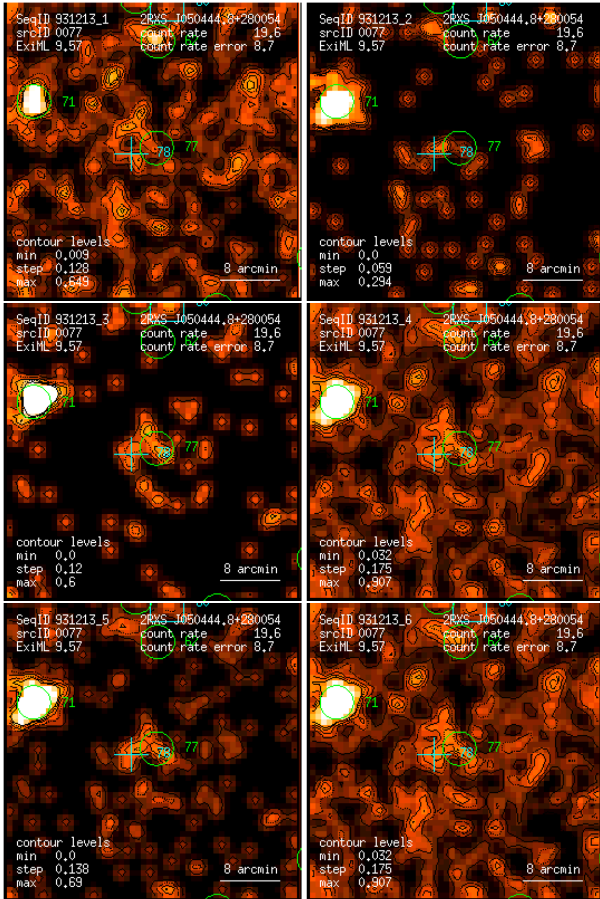
Figure 77: RASS 931213: detection 0077: band rate images, Gaussian filter: (1) PSPC channels 11 – 41, (2) 52 – 90, (3) 91 – 201, (4) 11 – 235, (5) 52 – 201, (6) 11 – 201. Broad band rates in counts/ks. Band rate contour levels in counts/ks/arcmin 2 .
