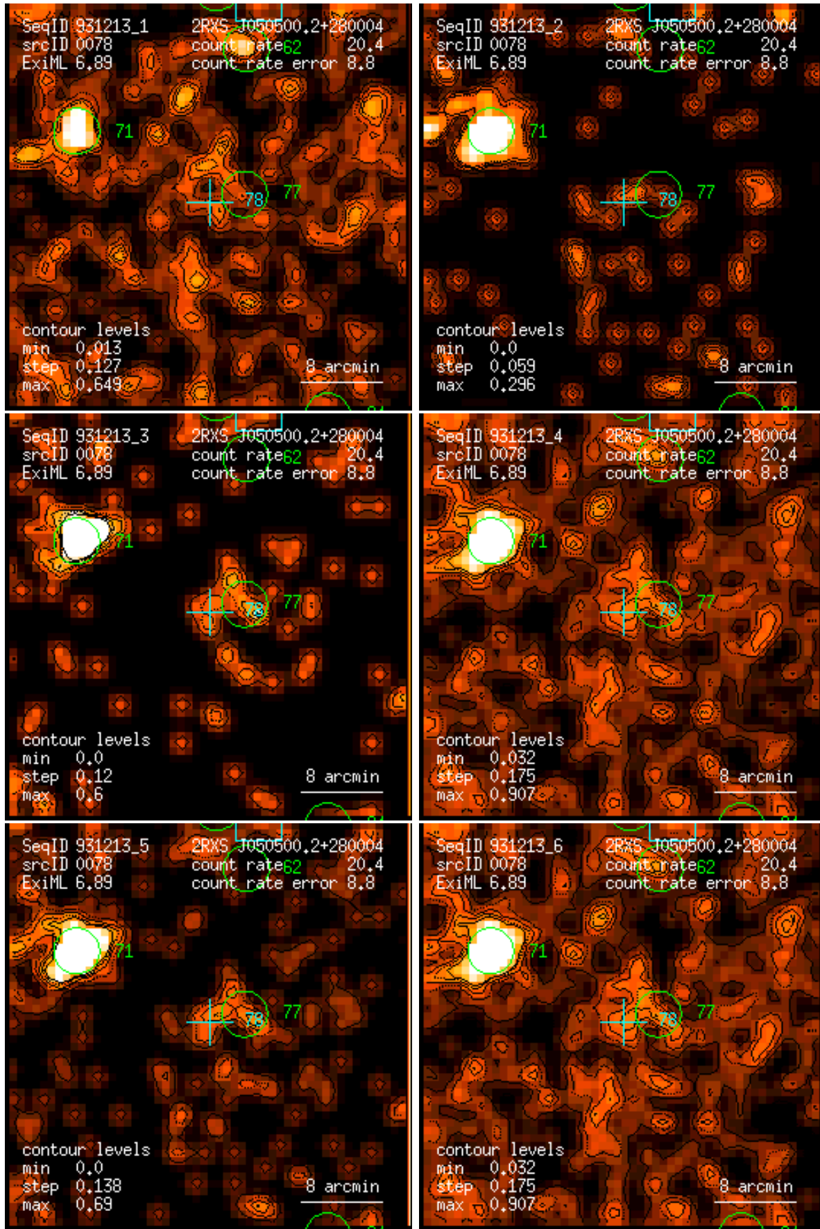
Figure 78: RASS 931213: detection 0078: band rate images, Gaussian filter: (1) PSPC channels 11 – 41, (2) 52 – 90, (3) 91 – 201, (4) 11 – 235, (5) 52 – 201, (6) 11 – 201. Broad band rates in counts/ks. Band rate contour levels in counts/ks/arcmin 2 .
