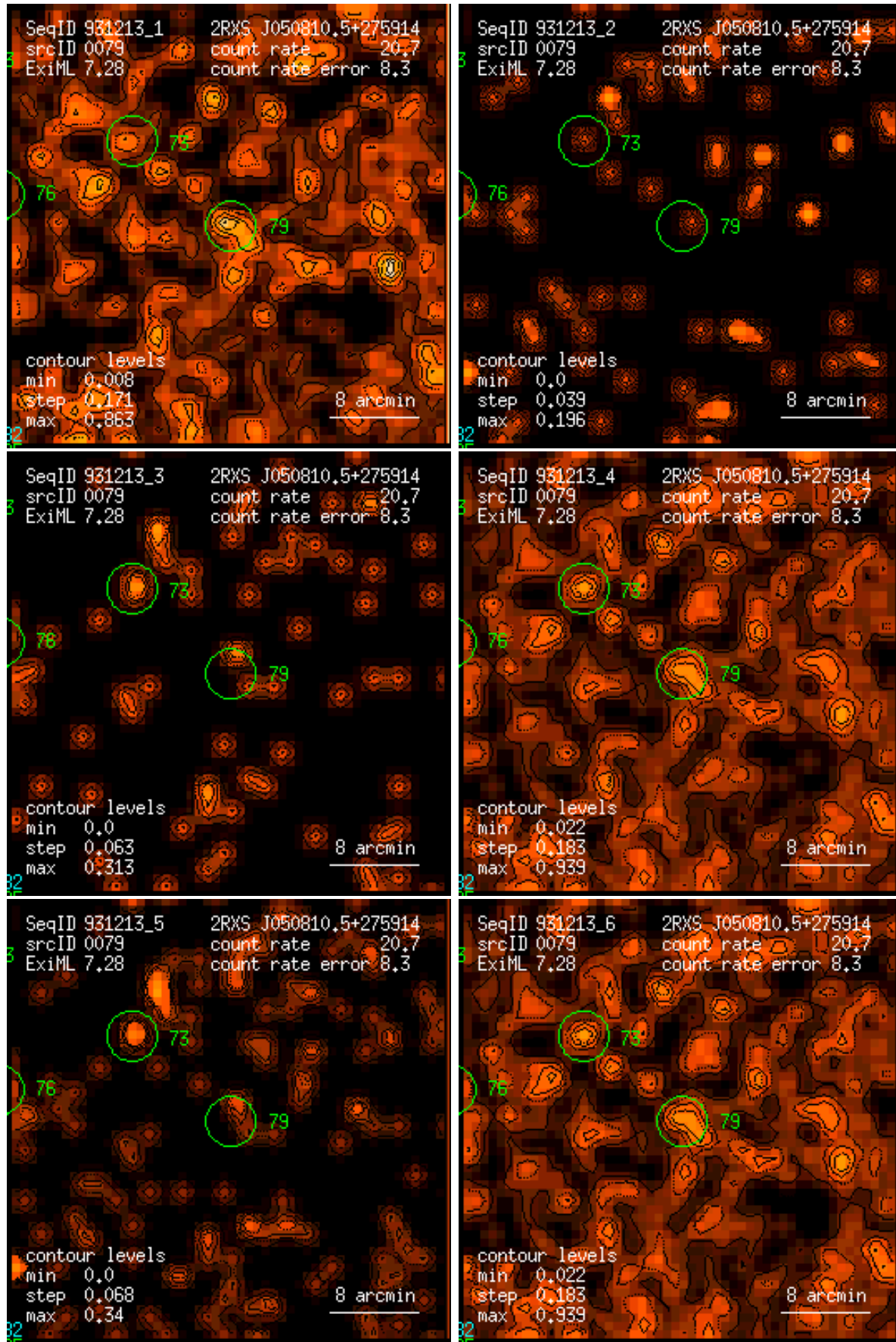
Figure 79: RASS 931213: detection 0079: band rate images, Gaussian filter: (1) PSPC channels 11 – 41, (2) 52 – 90, (3) 91 – 201, (4) 11 – 235, (5) 52 – 201, (6) 11 – 201. Broad band rates in counts/ks. Band rate contour levels in counts/ks/arcmin 2 .
