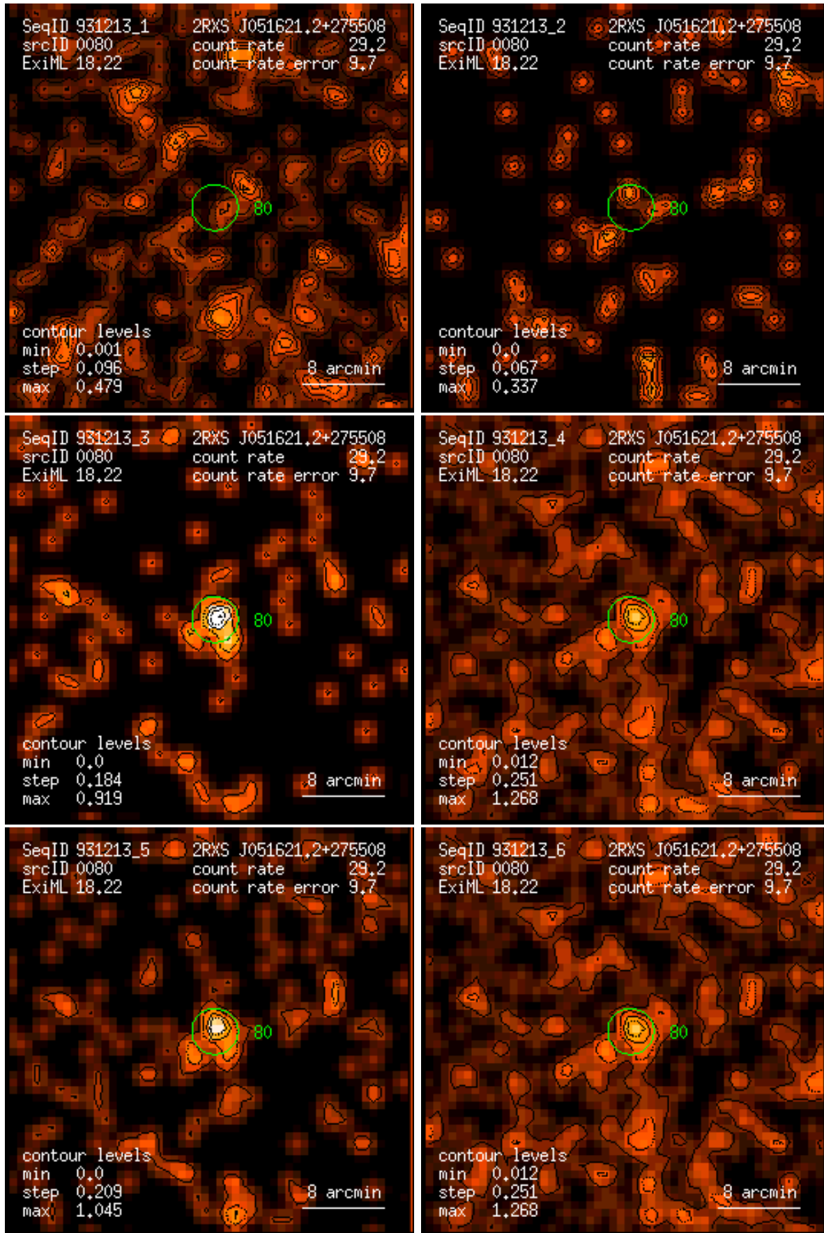
Figure 80: RASS 931213: detection 0080: band rate images, Gaussian filter: (1) PSPC channels 11 – 41, (2) 52 – 90, (3) 91 – 201, (4) 11 – 235, (5) 52 – 201, (6) 11 – 201. Broad band rates in counts/ks. Band rate contour levels in counts/ks/arcmin 2 .
