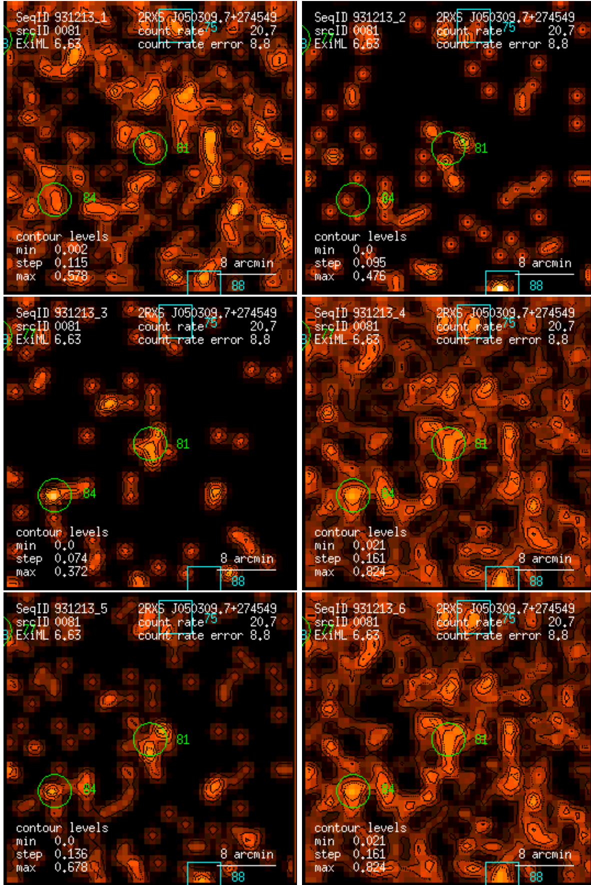
Figure 81: RASS 931213: detection 0081: band rate images, Gaussian filter: (1) PSPC channels 11 – 41, (2) 52 – 90, (3) 91 – 201, (4) 11 – 235, (5) 52 – 201, (6) 11 – 201. Broad band rates in counts/ks. Band rate contour levels in counts/ks/arcmin 2 .
