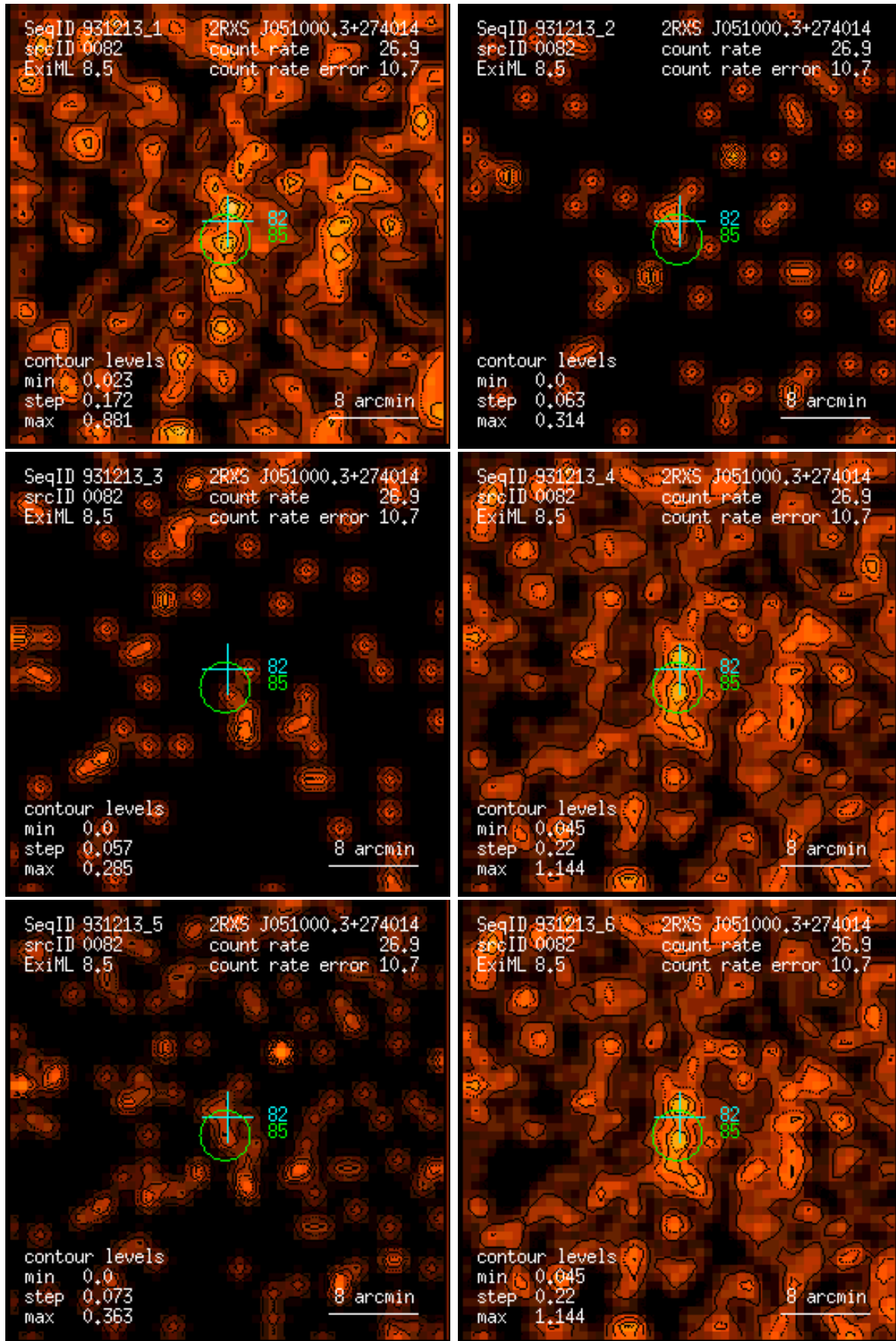
Figure 82: RASS 931213: detection 0082: band rate images, Gaussian filter: (1) PSPC channels 11 – 41, (2) 52 – 90, (3) 91 – 201, (4) 11 – 235, (5) 52 – 201, (6) 11 – 201. Broad band rates in counts/ks. Band rate contour levels in counts/ks/arcmin 2 .
