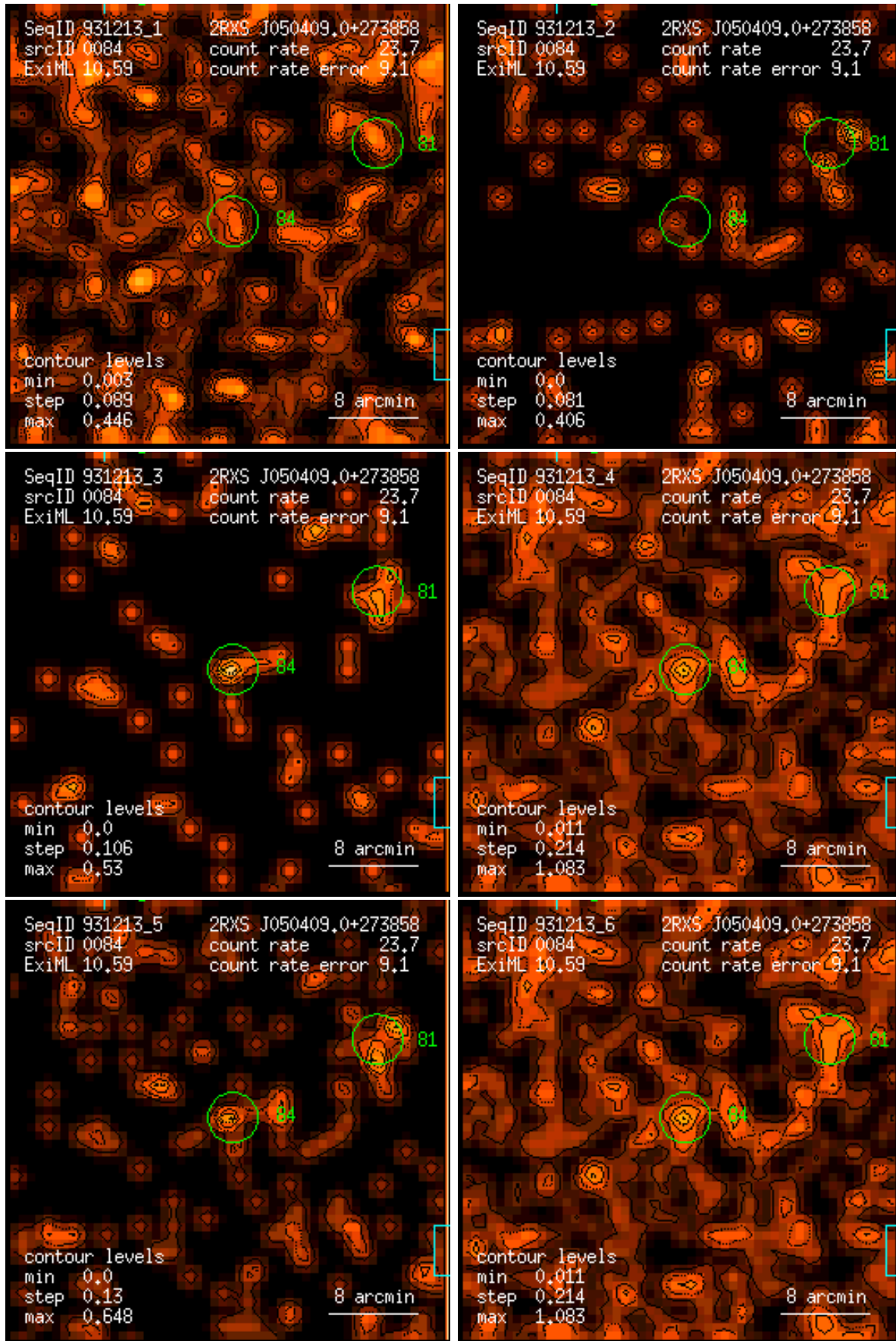
Figure 84: RASS 931213: detection 0084: band rate images, Gaussian filter: (1) PSPC channels 11 – 41, (2) 52 – 90, (3) 91 – 201, (4) 11 – 235, (5) 52 – 201, (6) 11 – 201. Broad band rates in counts/ks. Band rate contour levels in counts/ks/arcmin 2 .
