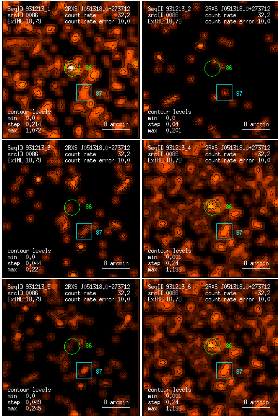
Figure 86: RASS 931213: detection 0086: band rate images, Gaussian filter: (1) PSPC channels 11 – 41, (2) 52 – 90, (3) 91 – 201, (4) 11 – 235, (5) 52 – 201, (6) 11 – 201. Broad band rates in counts/ks. Band rate contour levels in counts/ks/arcmin 2 .
