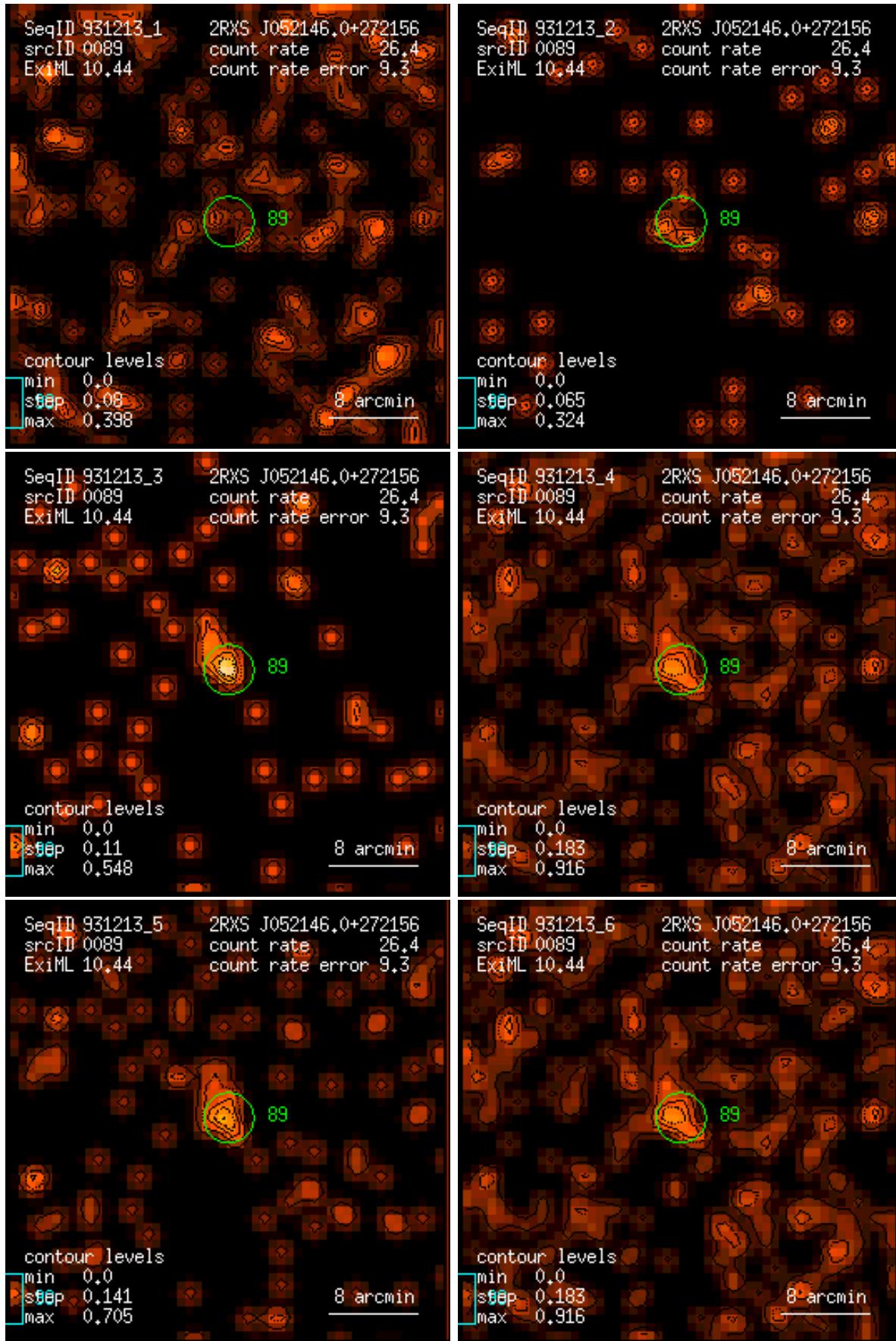
Figure 89: RASS 931213: detection 0089: band rate images, Gaussian filter: (1) PSPC channels 11 – 41, (2) 52 – 90, (3) 91 – 201, (4) 11 – 235, (5) 52 – 201, (6) 11 – 201. Broad band rates in counts/ks. Band rate contour levels in counts/ks/arcmin 2 .
