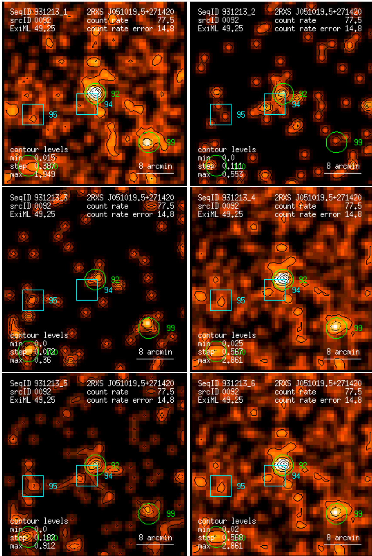
Figure 92: RASS 931213: detection 0092: band rate images, Gaussian filter: (1) PSPC channels 11 – 41, (2) 52 – 90, (3) 91 – 201, (4) 11 – 235, (5) 52 – 201, (6) 11 – 201. Broad band rates in counts/ks. Band rate contour levels in counts/ks/arcmin 2 .
