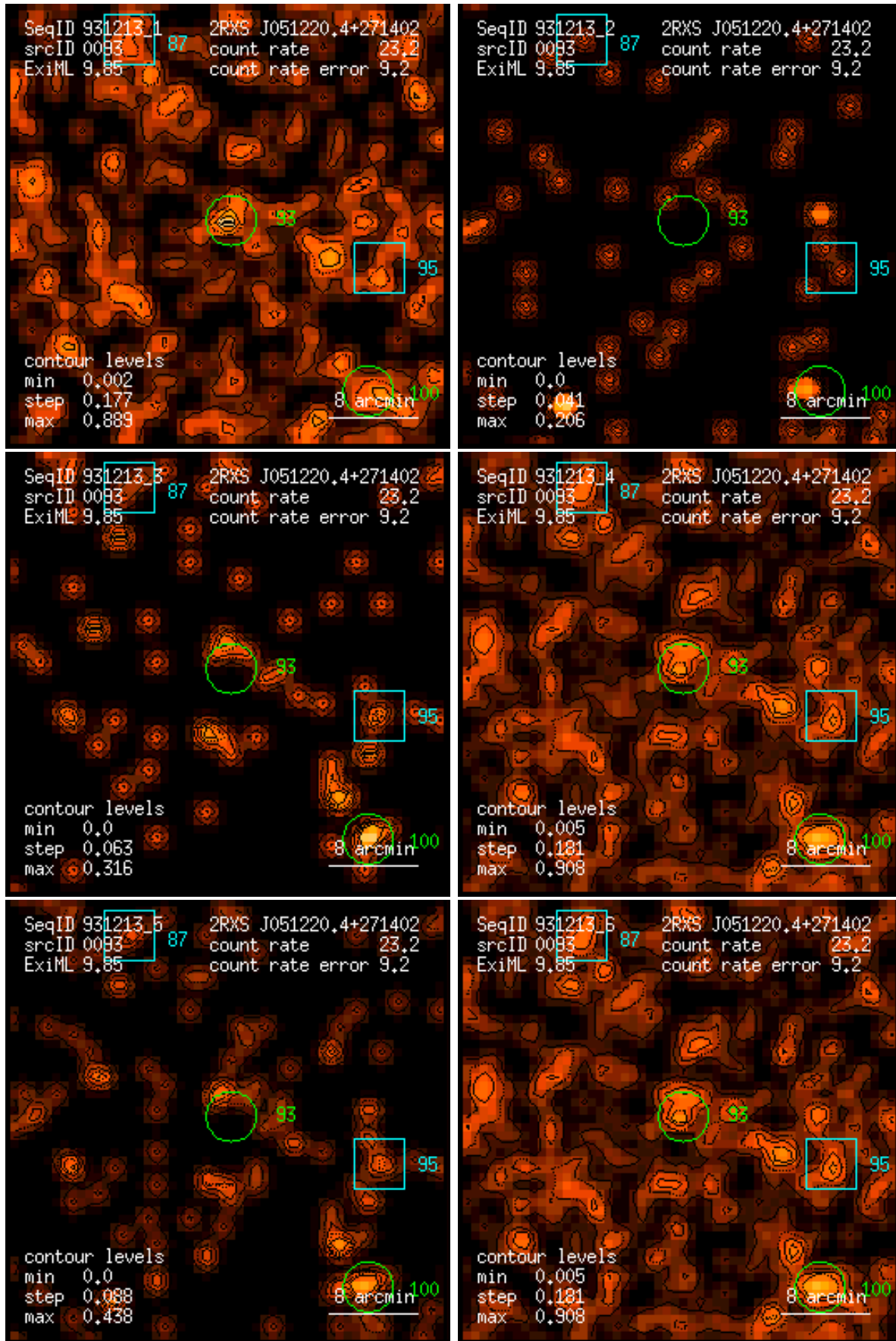
Figure 93: RASS 931213: detection 0093: band rate images, Gaussian filter: (1) PSPC channels 11 – 41, (2) 52 – 90, (3) 91 – 201, (4) 11 – 235, (5) 52 – 201, (6) 11 – 201. Broad band rates in counts/ks. Band rate contour levels in counts/ks/arcmin 2 .
