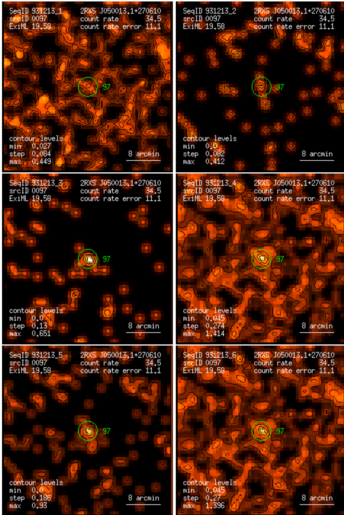
Figure 97: RASS 931213: detection 0097: band rate images, Gaussian filter: (1) PSPC channels 11 – 41, (2) 52 – 90, (3) 91 – 201, (4) 11 – 235, (5) 52 – 201, (6) 11 – 201. Broad band rates in counts/ks. Band rate contour levels in counts/ks/arcmin 2 .
