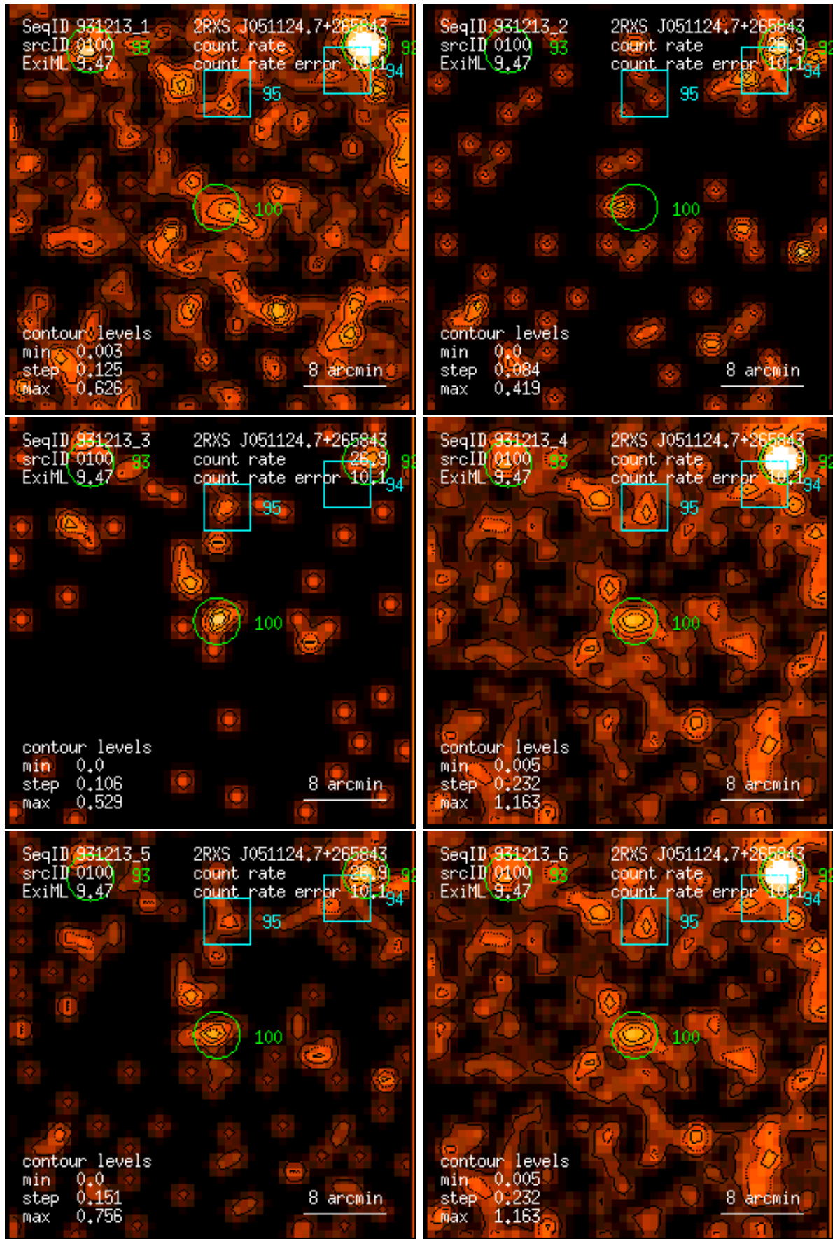
Figure 100: RASS 931213: detection 0100: band rate images, Gaussian filter: (1) PSPC channels 11 – 41, (2) 52 – 90, (3) 91 – 201, (4) 11 – 235, (5) 52 – 201, (6) 11 – 201. Broad band rates in counts/ks. Band rate contour levels in counts/ks/arcmin 2 .
