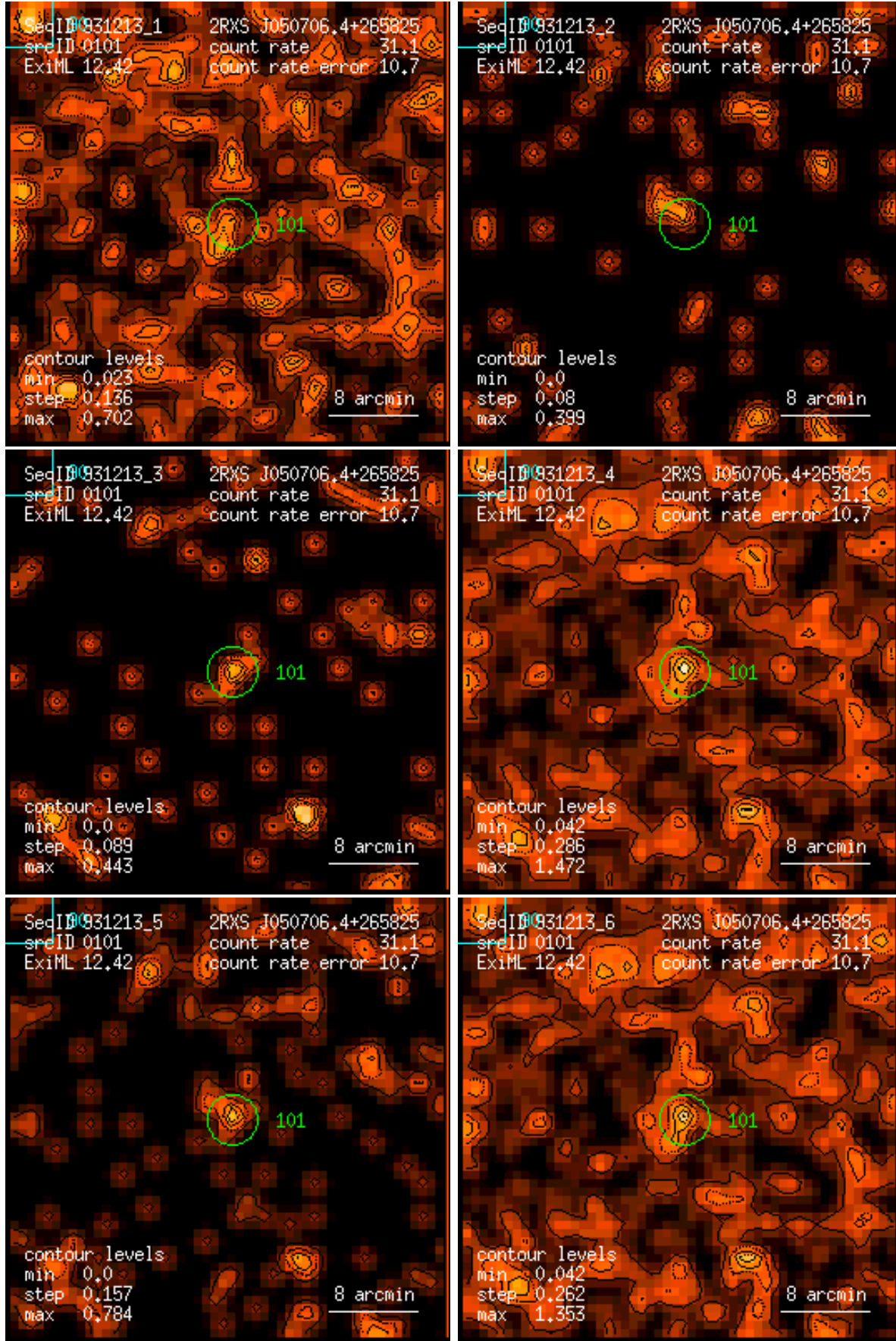
Figure 101: RASS 931213: detection 0101: band rate images, Gaussian filter: (1) PSPC channels 11 – 41, (2) 52 – 90, (3) 91 – 201, (4) 11 – 235, (5) 52 – 201, (6) 11 – 201. Broad band rates in counts/ks. Band rate contour levels in counts/ks/arcmin 2 .
