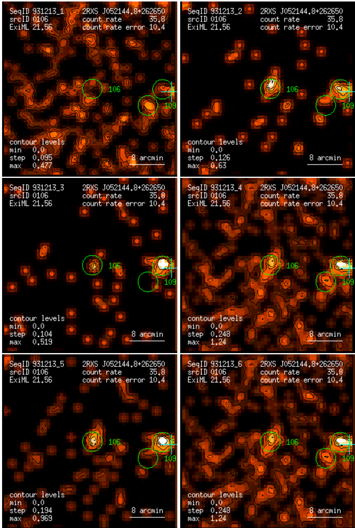
Figure 106: RASS 931213: detection 0106: band rate images, Gaussian filter: (1) PSPC channels 11 – 41, (2) 52 – 90, (3) 91 – 201, (4) 11 – 235, (5) 52 – 201, (6) 11 – 201. Broad band rates in counts/ks. Band rate contour levels in counts/ks/arcmin 2 .
