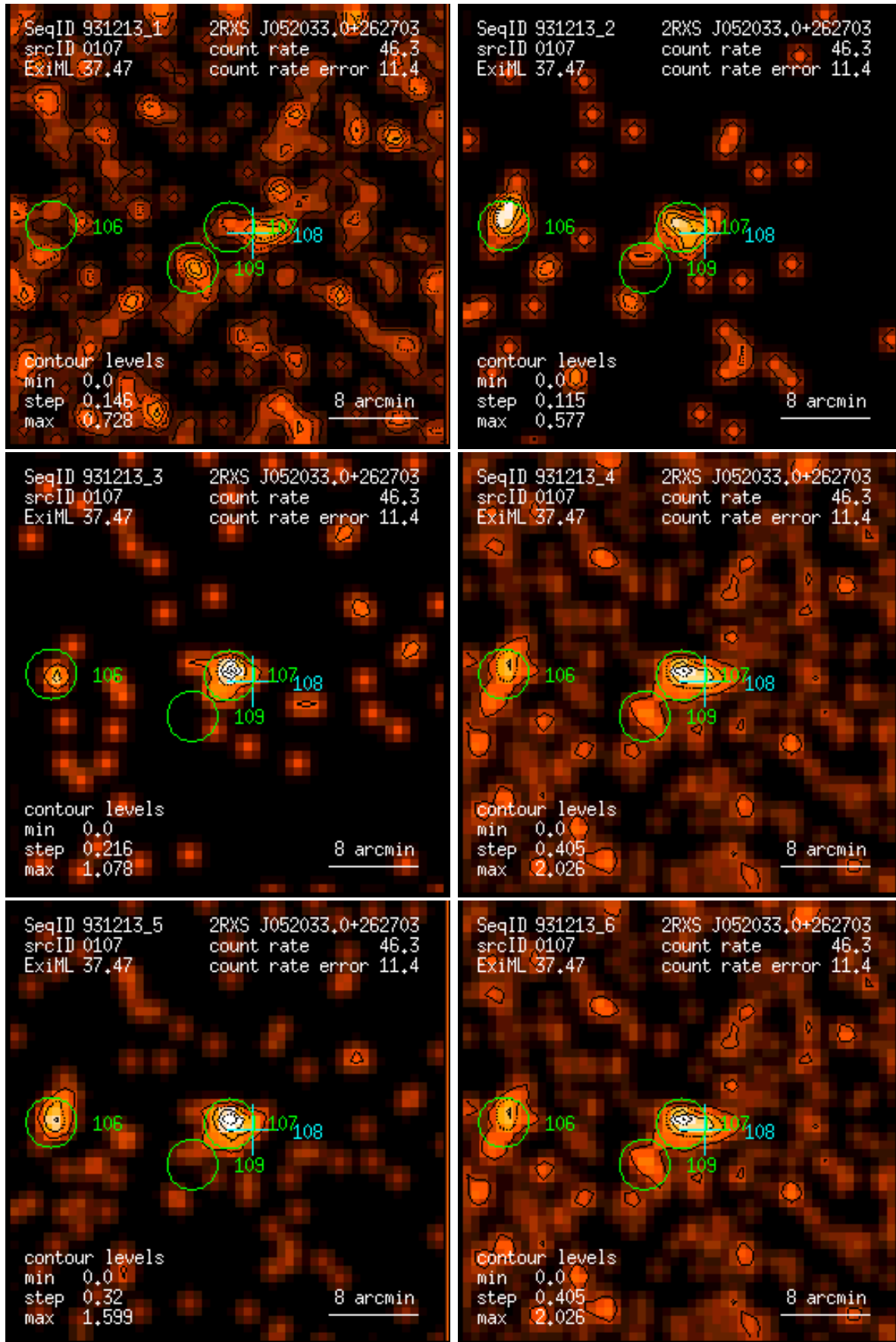
Figure 107: RASS 931213: detection 0107: band rate images, Gaussian filter: (1) PSPC channels 11 – 41, (2) 52 – 90, (3) 91 – 201, (4) 11 – 235, (5) 52 – 201, (6) 11 – 201. Broad band rates in counts/ks. Band rate contour levels in counts/ks/arcmin 2 .
