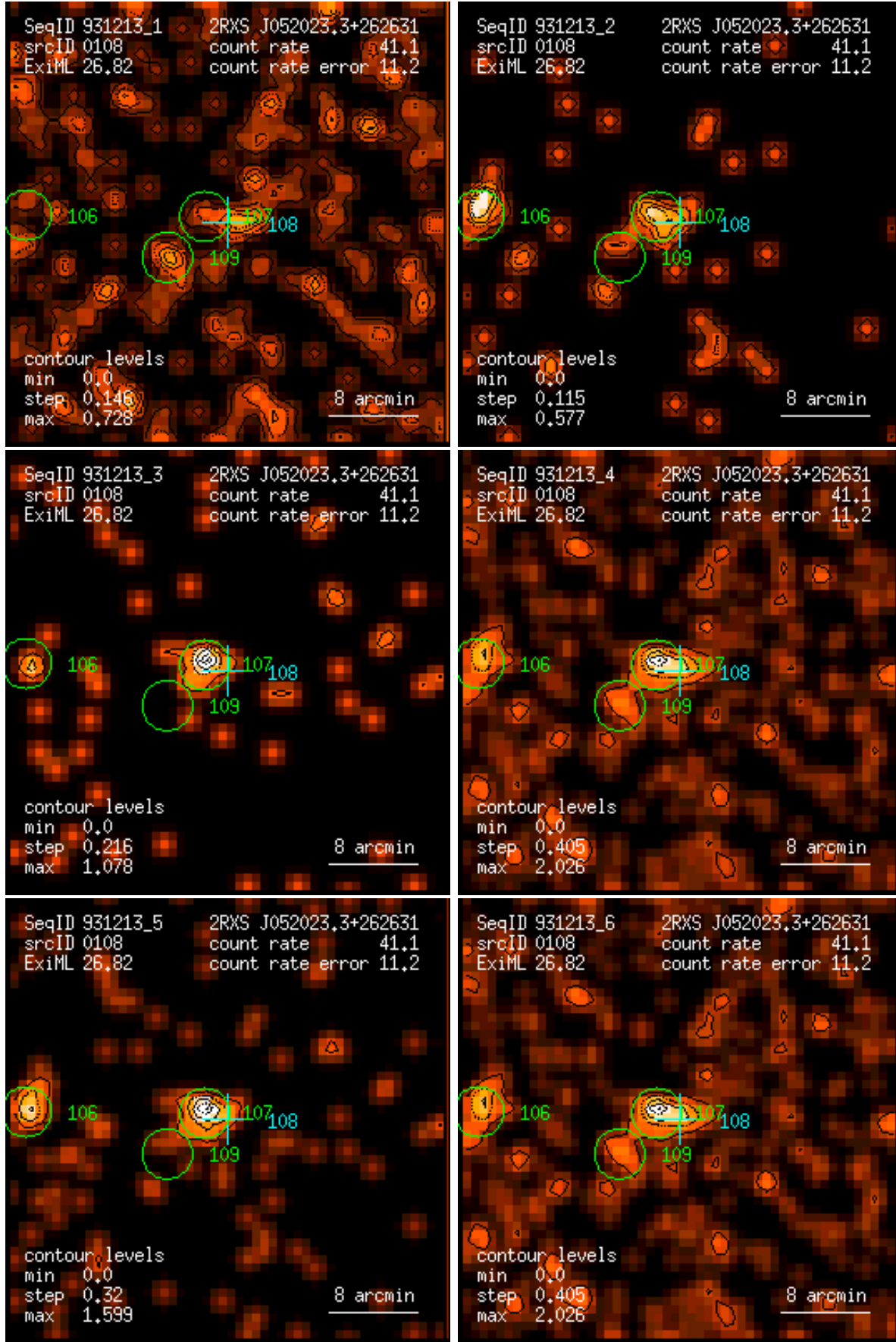
Figure 108: RASS 931213: detection 0108: band rate images, Gaussian filter: (1) PSPC channels 11 – 41, (2) 52 – 90, (3) 91 – 201, (4) 11 – 235, (5) 52 – 201, (6) 11 – 201. Broad band rates in counts/ks. Band rate contour levels in counts/ks/arcmin 2 .
