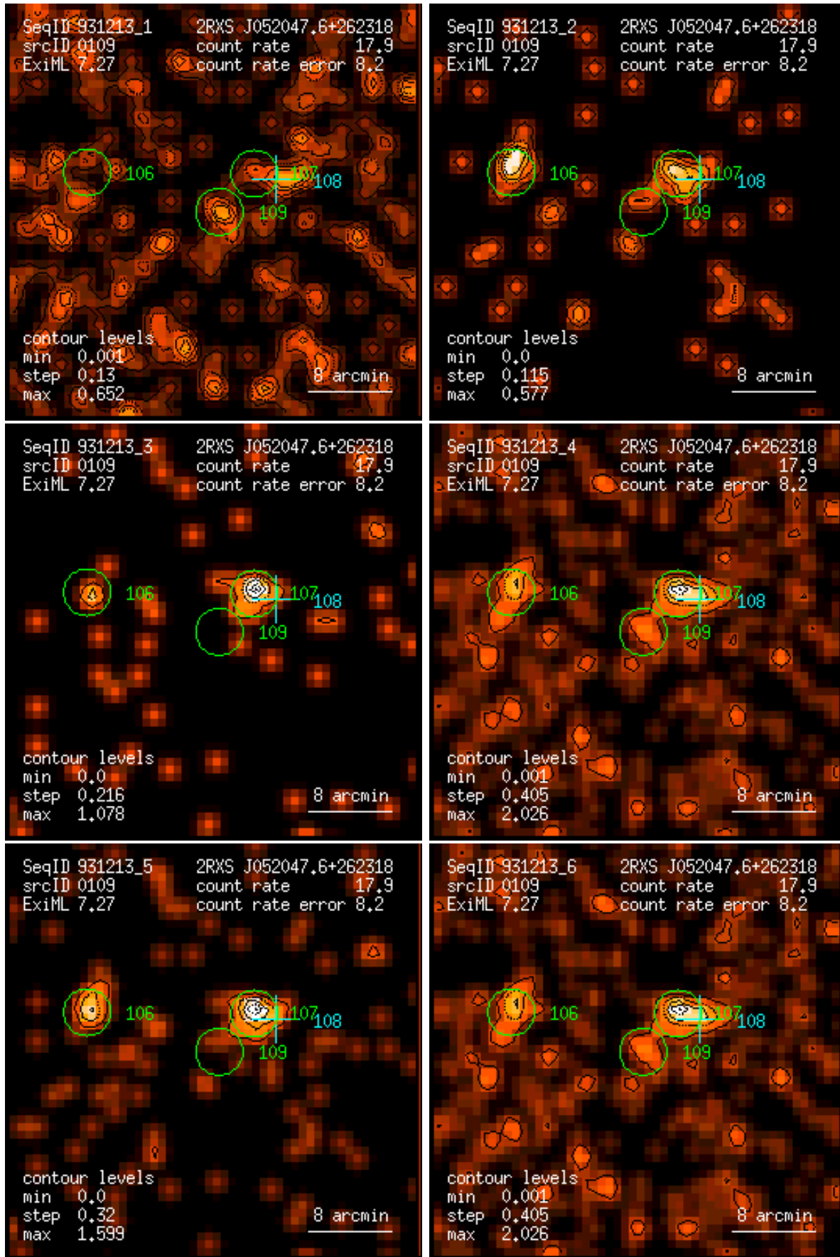
Figure 109: RASS 931213: detection 0109: band rate images, Gaussian filter: (1) PSPC channels 11 – 41, (2) 52 – 90, (3) 91 – 201, (4) 11 – 235, (5) 52 – 201, (6) 11 – 201. Broad band rates in counts/ks. Band rate contour levels in counts/ks/arcmin 2 .
