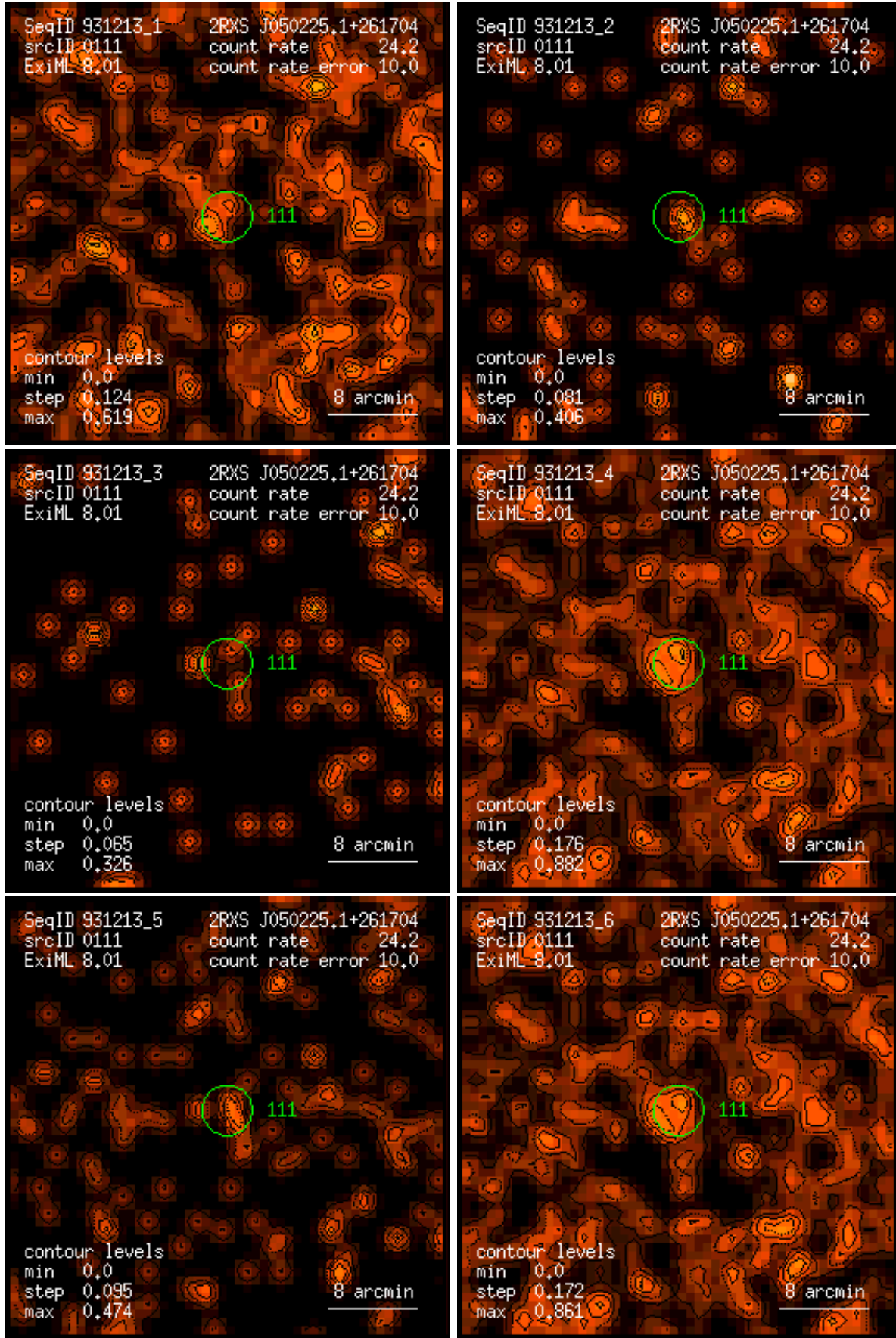
Figure 111: RASS 931213: detection 0111: band rate images, Gaussian filter: (1) PSPC channels 11 – 41, (2) 52 – 90, (3) 91 – 201, (4) 11 – 235, (5) 52 – 201, (6) 11 – 201. Broad band rates in counts/ks. Band rate contour levels in counts/ks/arcmin 2 .
