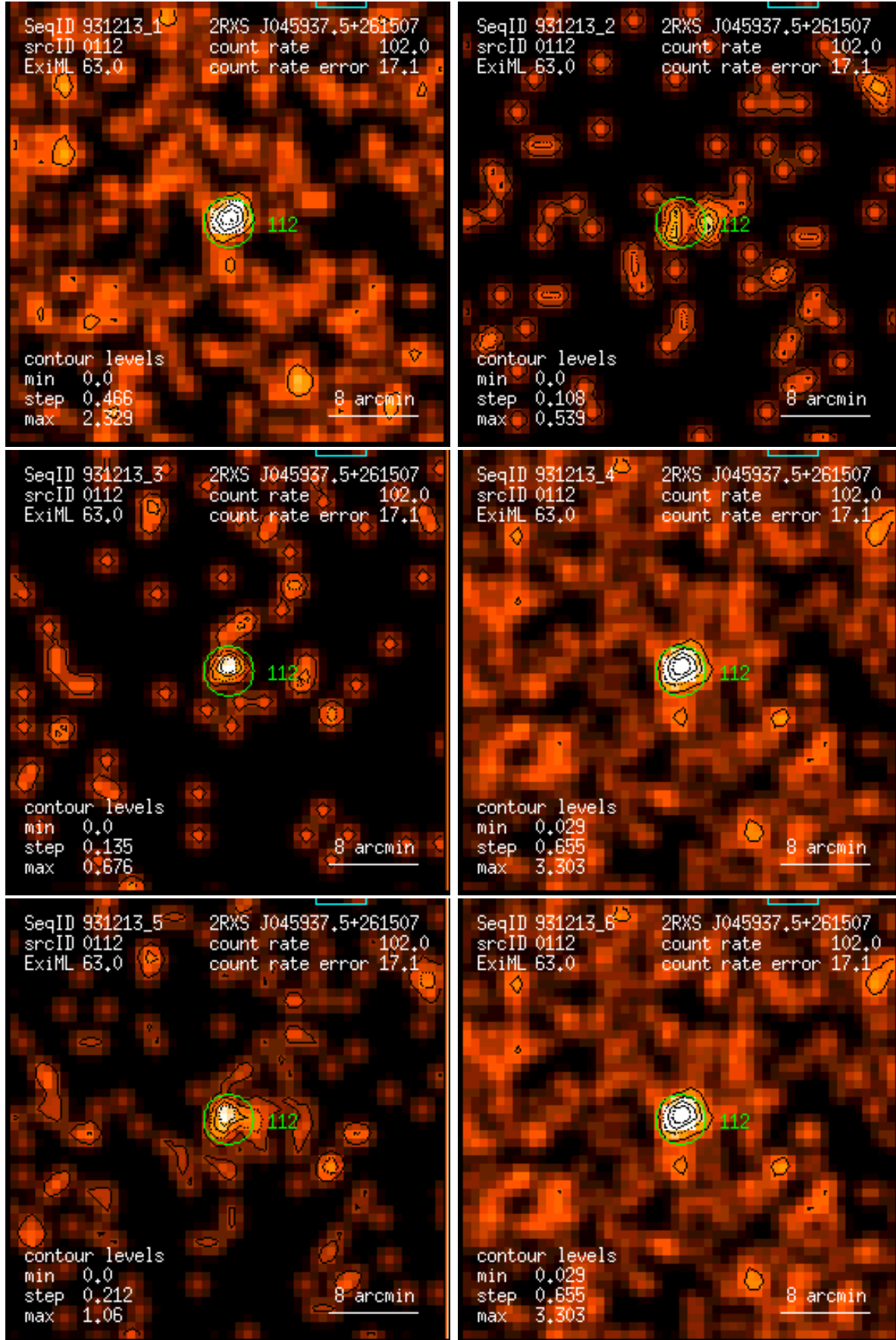
Figure 112: RASS 931213: detection 0112: band rate images, Gaussian filter: (1) PSPC channels 11 – 41, (2) 52 – 90, (3) 91 – 201, (4) 11 – 235, (5) 52 – 201, (6) 11 – 201. Broad band rates in counts/ks. Band rate contour levels in counts/ks/arcmin 2 .
